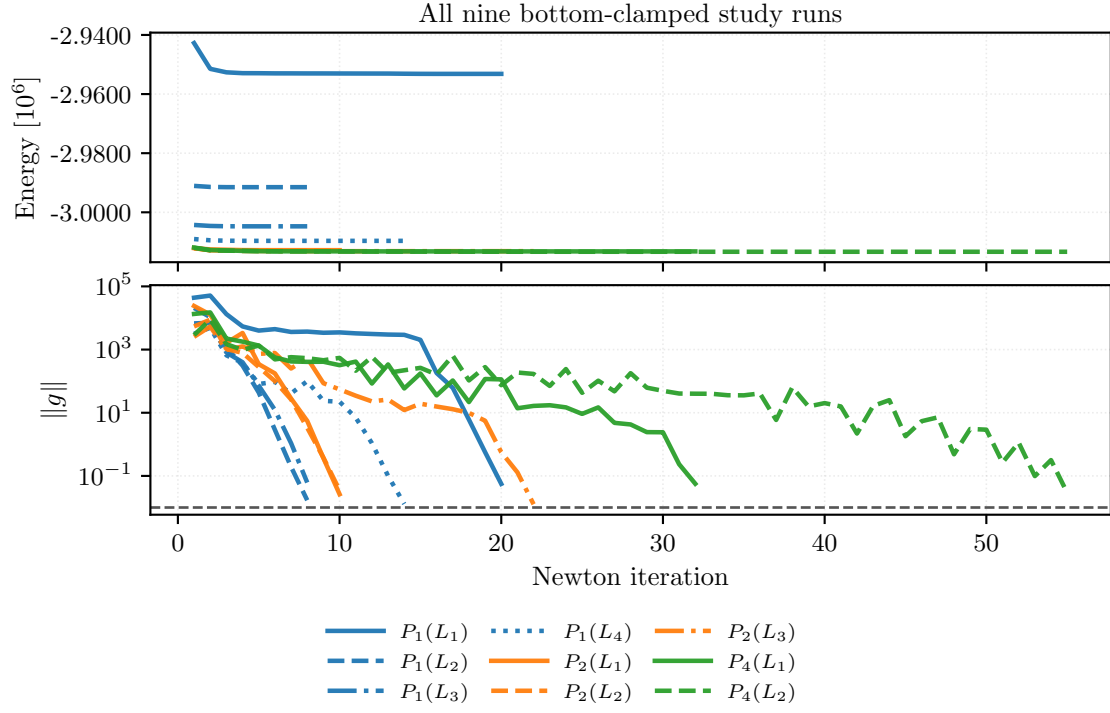
Figure 15: Newton-history convergence for all nine completed bottom-clamped Plasticity3D study runs at \lambda_{sr} = 1.55 . The upper panel shows the value of the algorithmic surrogate from equation (22); the lower panel shows the gradient norm used as the nonlinear stopping metric, with color indicating degree and line style indicating mesh level.
