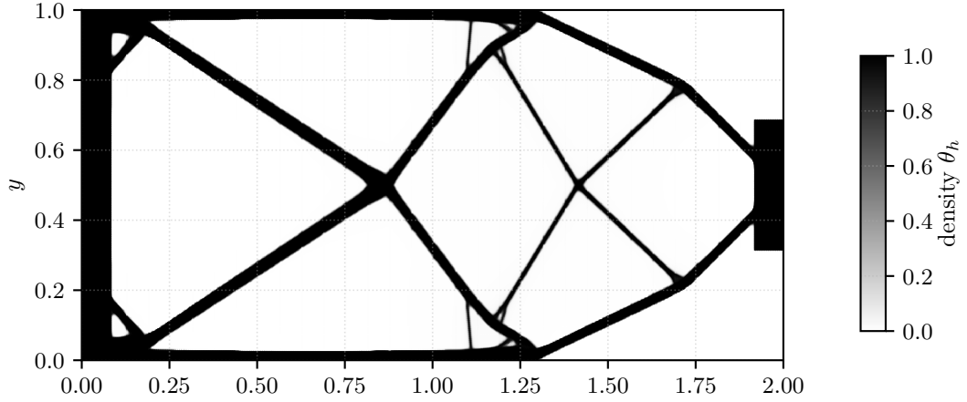
Figure 17: Representative final density field for the maintained parallel topology benchmark.
