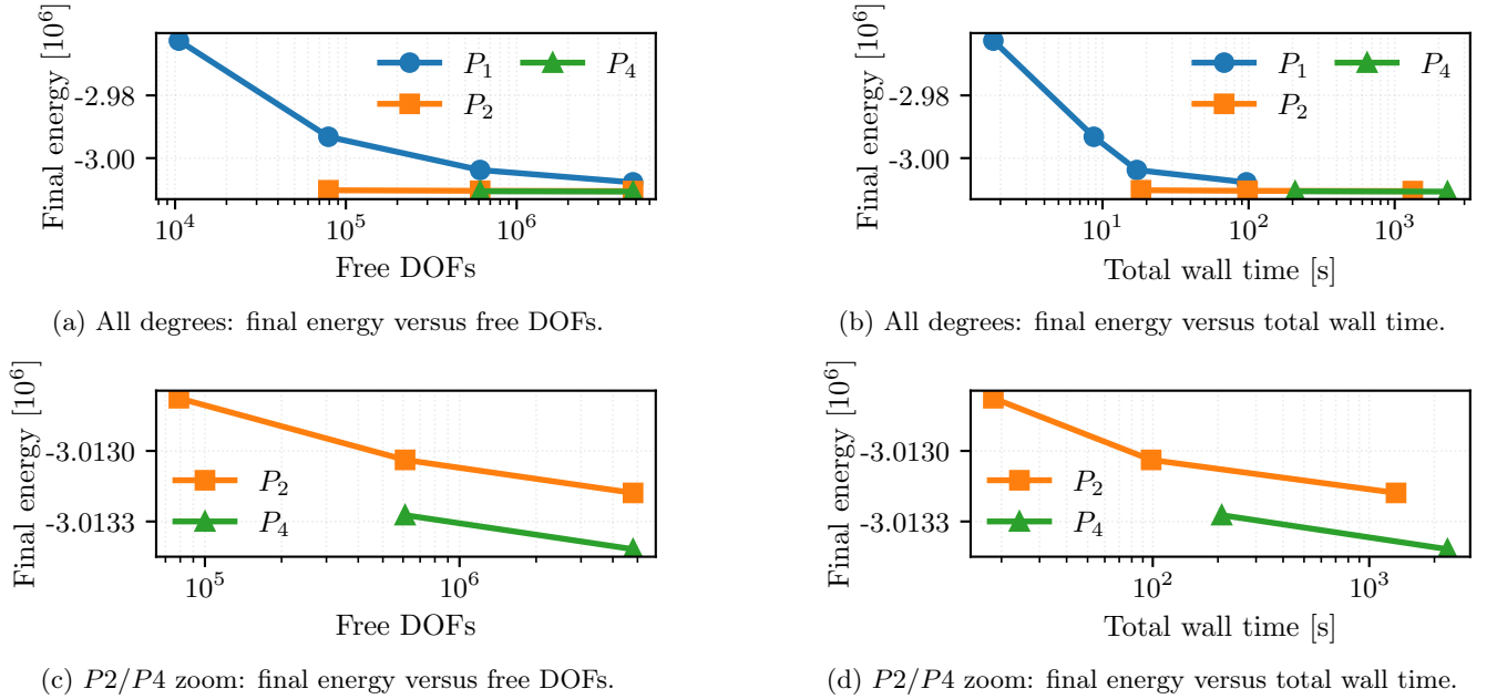
Figure 26: Corrected glued-bottom Plasticity3D degree-versus-resolution study at \lambda_{\text{sr}} = 1.55 . The top row shows the full P_1/P_2/P_4 comparison, while the bottom row zooms to P_2/P_4 so the near-overlap hidden by the coarse P_1 points becomes visible. The left column plots final values of equation (21) against free DOFs; the right column plots the same converged energies against end-to-end wall time. All timings are fair 32-rank runs.
