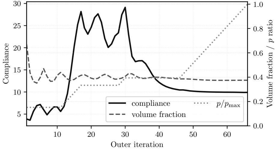
Figure 18: Objective-history view for the reduced topology objective equation (32), with compliance on the left axis and volume fraction plus the continuation schedule in p on the right axis.
