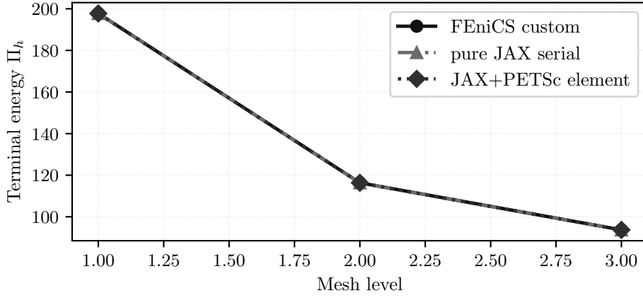
Figure 11: Final discrete energies along the stationary sequence equation (14) across the selected mesh hierarchy. The comparison is less about exact equality than about tracking the same 24-step trajectory consistently.
