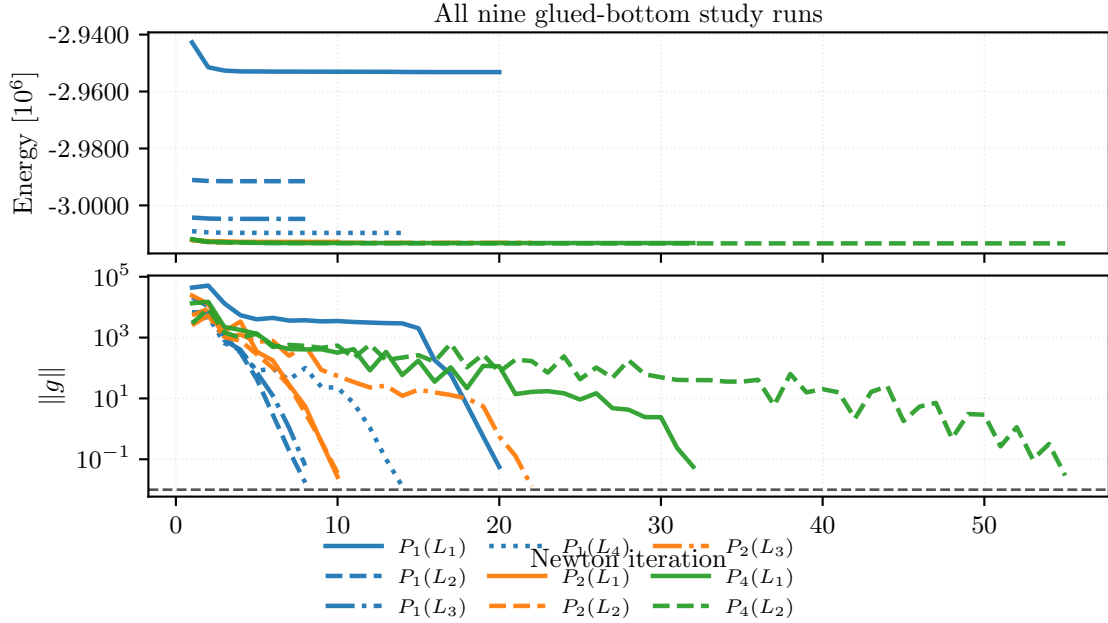
Figure 15: Newton-history convergence for all nine completed corrected glued-bottom Plasticity3D study runs at \lambda_{\text{sr}} = 1.55 . The upper panel shows the value of the algorithmic surrogate from equation (21); the lower panel shows the gradient norm used as the nonlinear stopping metric, with color indicating degree and line style indicating mesh level.
