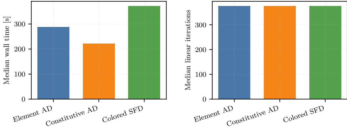
Figure 25: Locked Plasticity3D derivative-route ablation on P_4(L_1) , \lambda_{\text{sr}} = 1.5 , and 8 MPI ranks.
