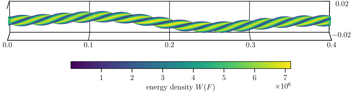
Figure 10: Representative finite-strain hyperelastic state, colored by the density W entering (13).
