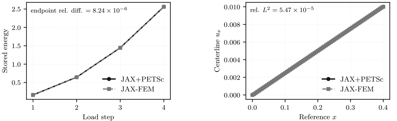
(a) Endpoint energy over the matched displacement schedule.
