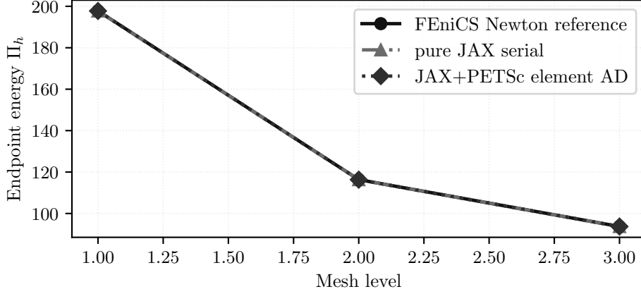
Figure 11: Final discrete energies along the stationary sequence (16) across the selected mesh hierarchy. The comparison records completion of the same 24-step schedule and comparable endpoint energies; this figure does not assess trajectory-level agreement.
