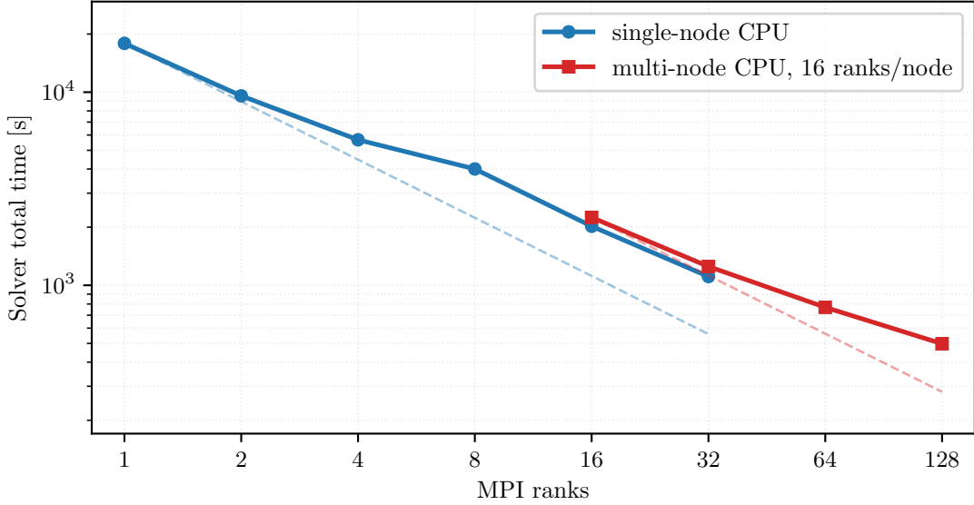
Figure 28: Single-node and multi-node CPU converged scaling for the bottom-clamped Plasticity3D P_4(L_2) case at \lambda_{\text{sr}} = 1.55 . Dashed references are ideal 1/r lines anchored separately to the first point of each CPU setting.
