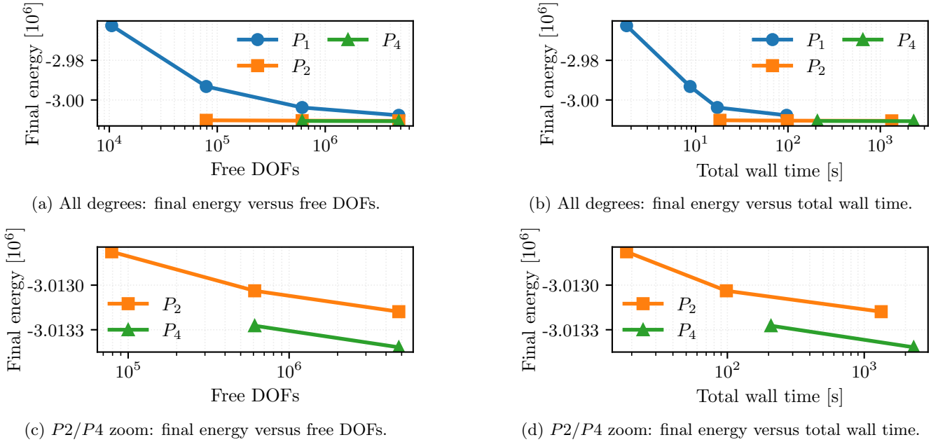
Figure 26: Corrected glued-bottom maintained Plasticity3D degree-versus-resolution study at \lambda_{\text{sr}} = 1.55 . The top row shows the full P_1/P_2/P_4 comparison, while the bottom row zooms to P_2/P_4 so the near-overlap hidden by the coarse P_1 points becomes visible. The left column plots final values of equation (22) against free DOFs; the right column plots the same converged energies against end-to-end wall time. All timings are fair 32-rank maintained runs.
