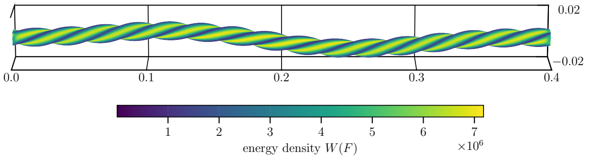
Figure 10: Representative finite-strain hyperelastic state, colored by the energy density in equation (12).
