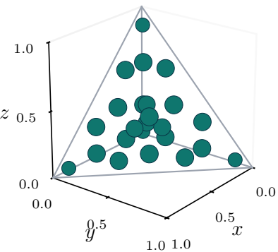
q24 (24 pts)
