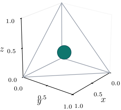
q24 (24 pts)
