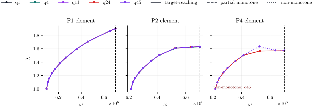
Figure 2: Continuation curves grouped by element family. The dashed vertical line marks the shared target \omega_{\text{final}} . Solid curves reached the shared target monotonically, while dashed curves denote monotone partial branches if a watchdog abort occurred before the target. Rules with no monotone branch are listed inside the affected panel.
