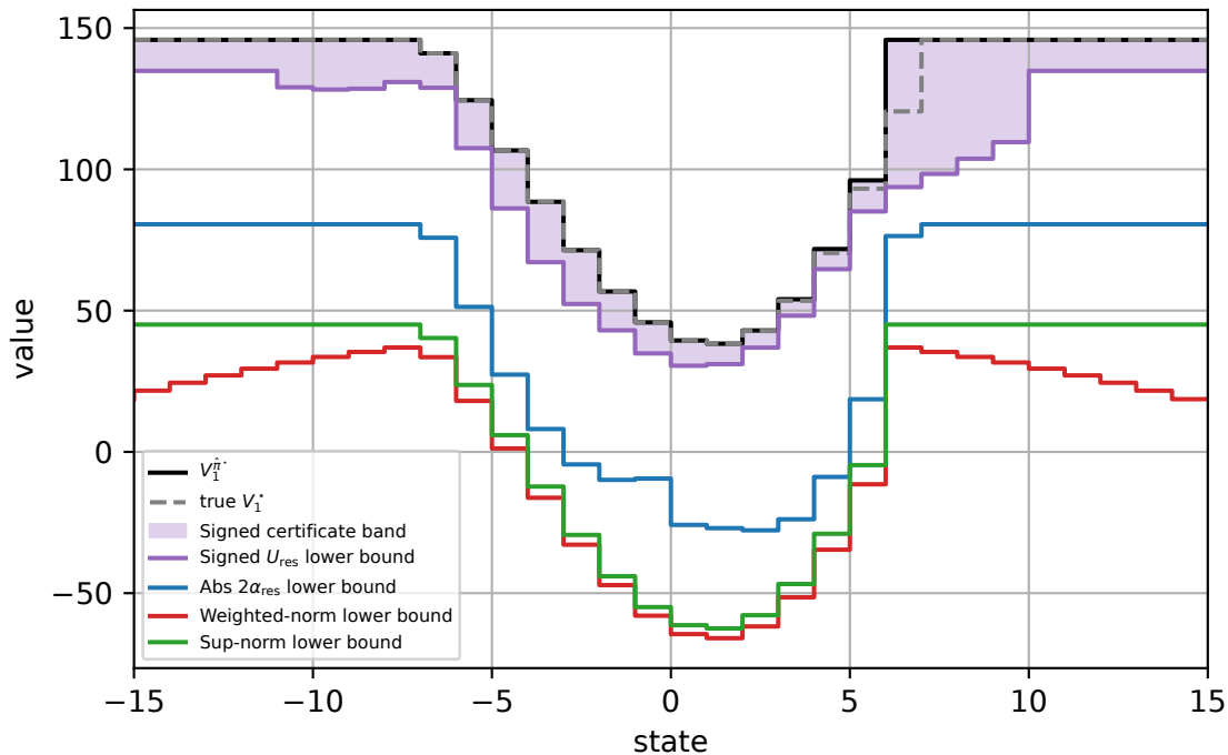
Signed U_{\text{res}} vs abs and weighted-norm: lower bound on V^*
