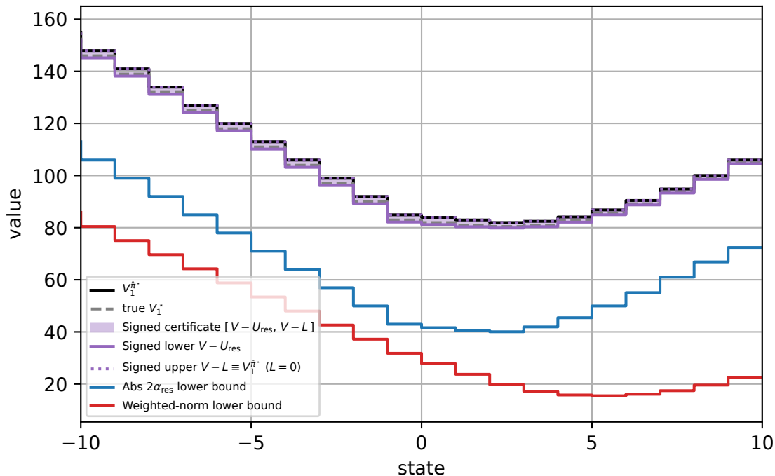
Signed two-sided certificate on V^* (Thm 3) vs abs \& weighted-norm
