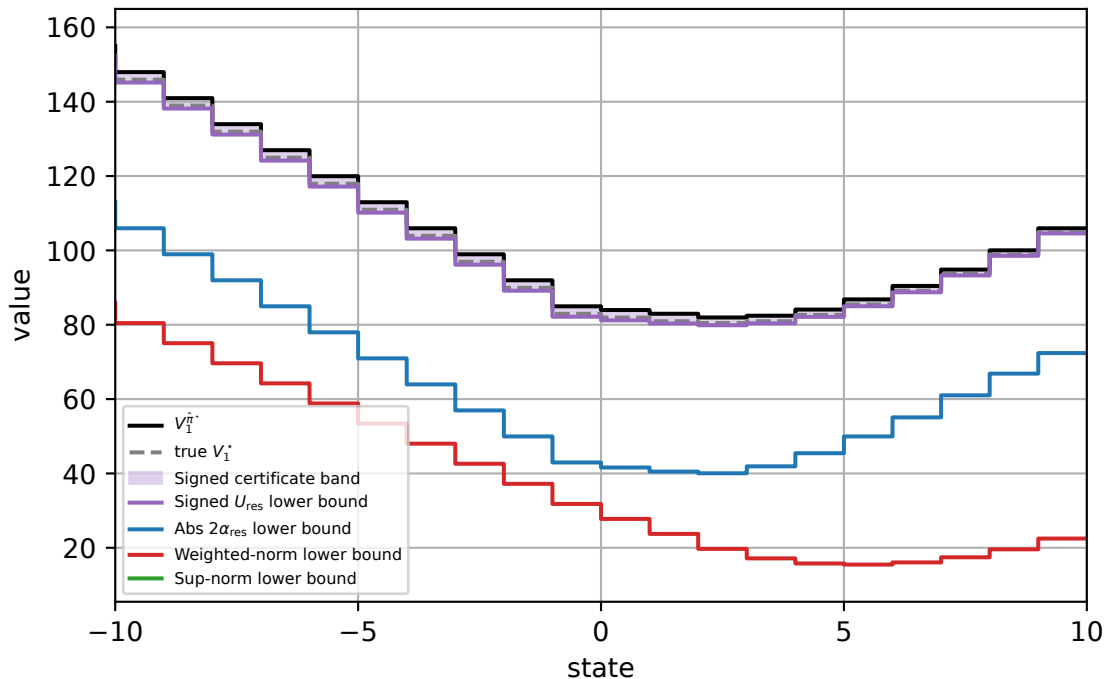
Signed U_{\text{res}} vs abs \& weighted-norm: lower bound on V^*
