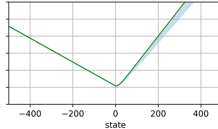
Sample-path abs ( 2\alpha_{\text{res}} , FH)
