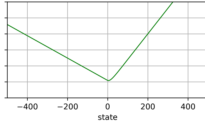
Sample-path signed ( U_{\text{res}} , FH)
