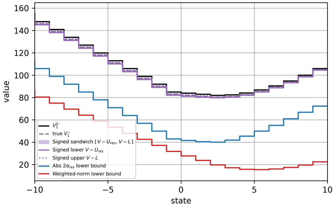
Signed (upper \& lower) sandwich on V^* vs abs \& weighted-norm
