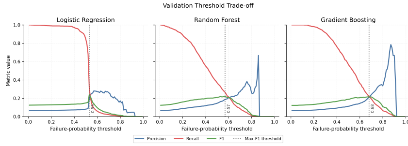
Figure 8: Validation precision, recall, and failed-class F1 across candidate thresholds. The figure uses validation predictions only.
