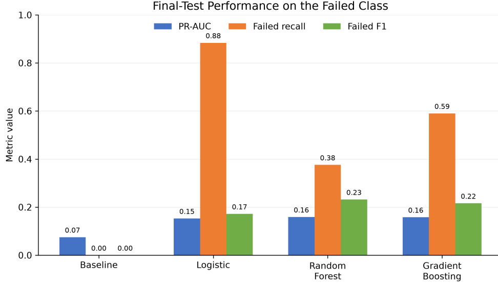
Figure 3: Final-test performance for the failed class. PR-AUC refers to average precision. The values come from the fixed held-out test set.
