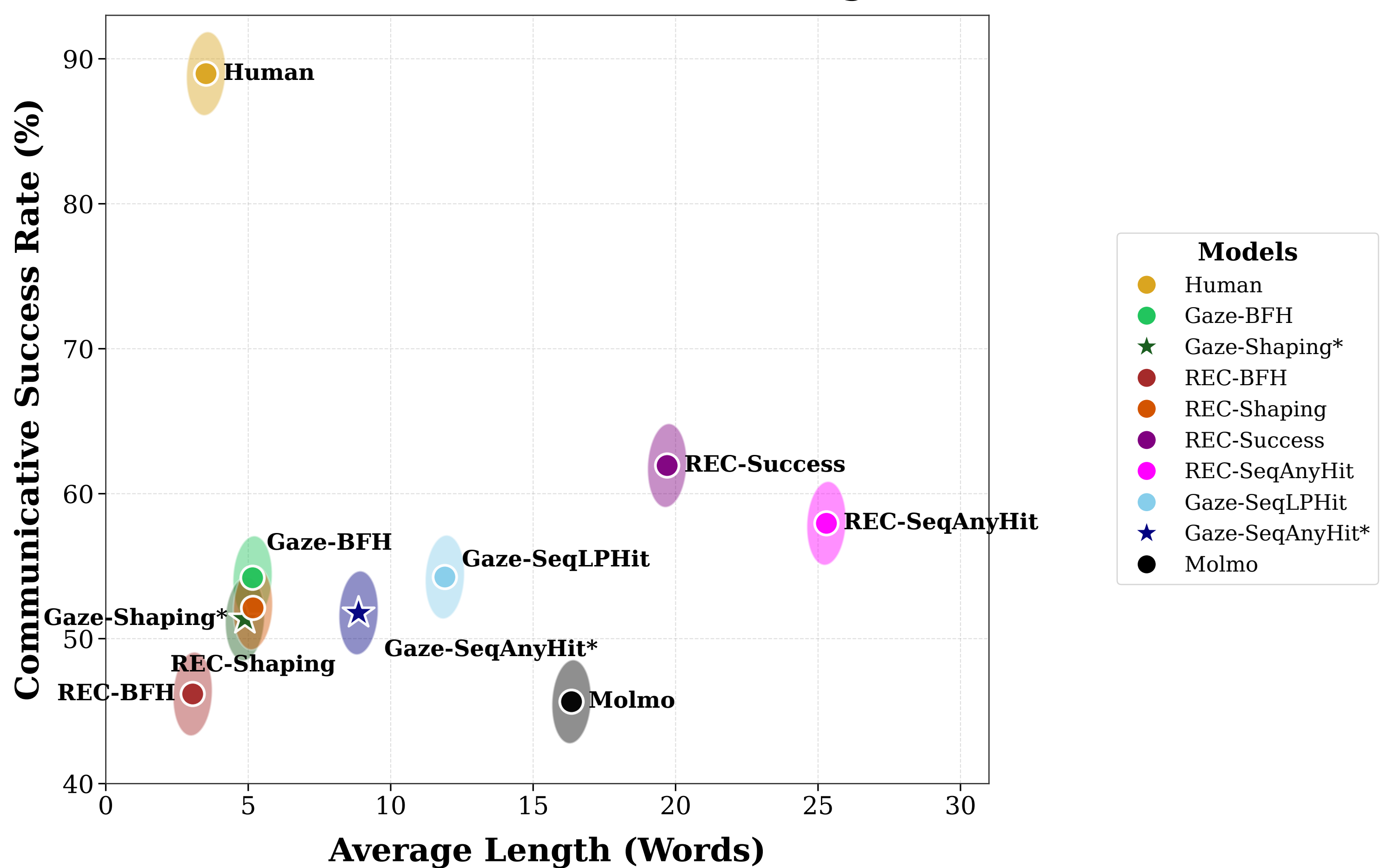
QwenVL Listener (Dataset Average)
