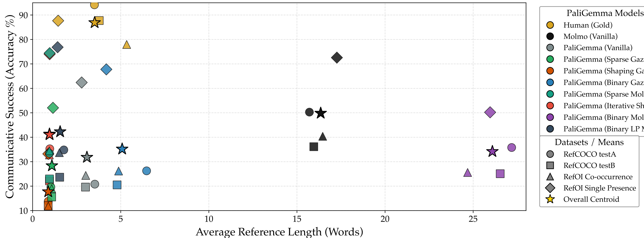
PaliGemma Ablations: Referential Efficiency (QwenVL Listener)
