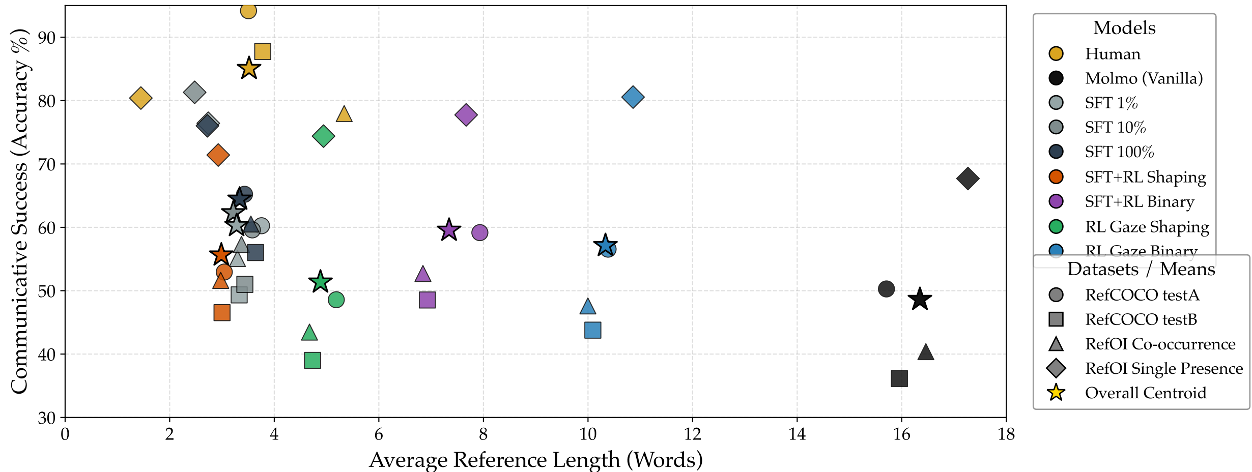
Efficiency Trade-off: SFT vs. RL & Gaze Models (QwenVL)
