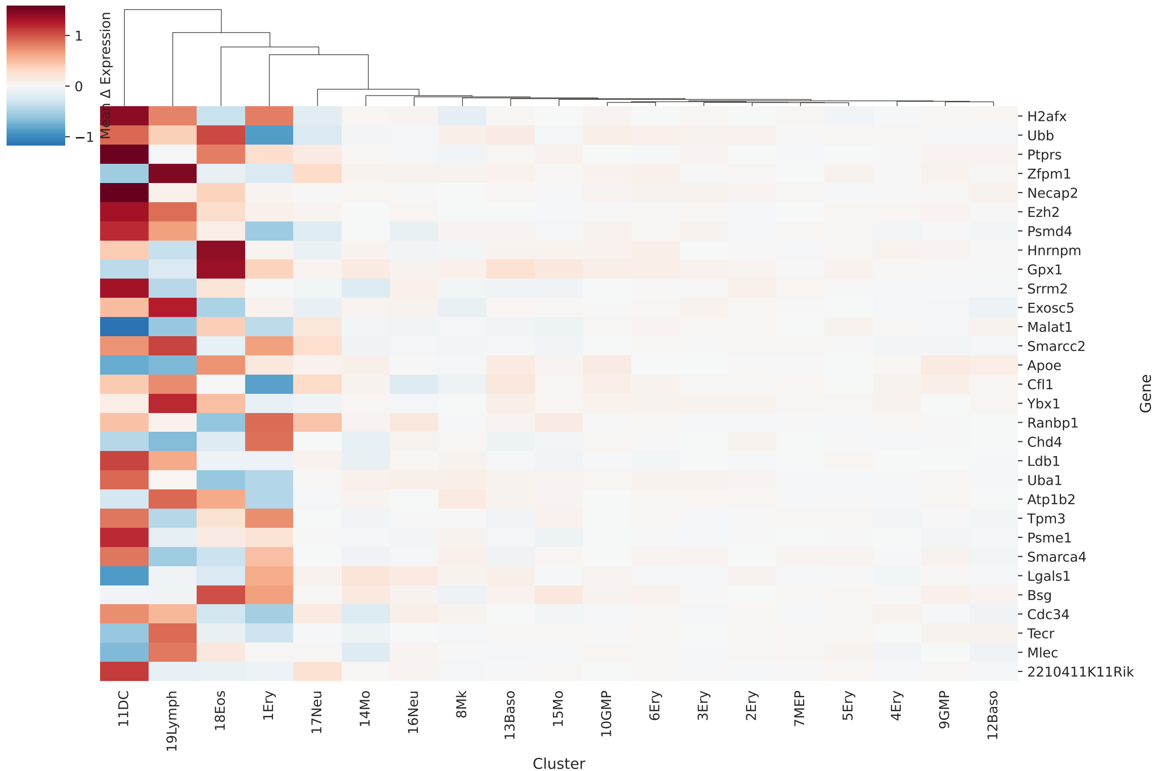
Gata1 OE (ODE) — perturbation effect heatmap
