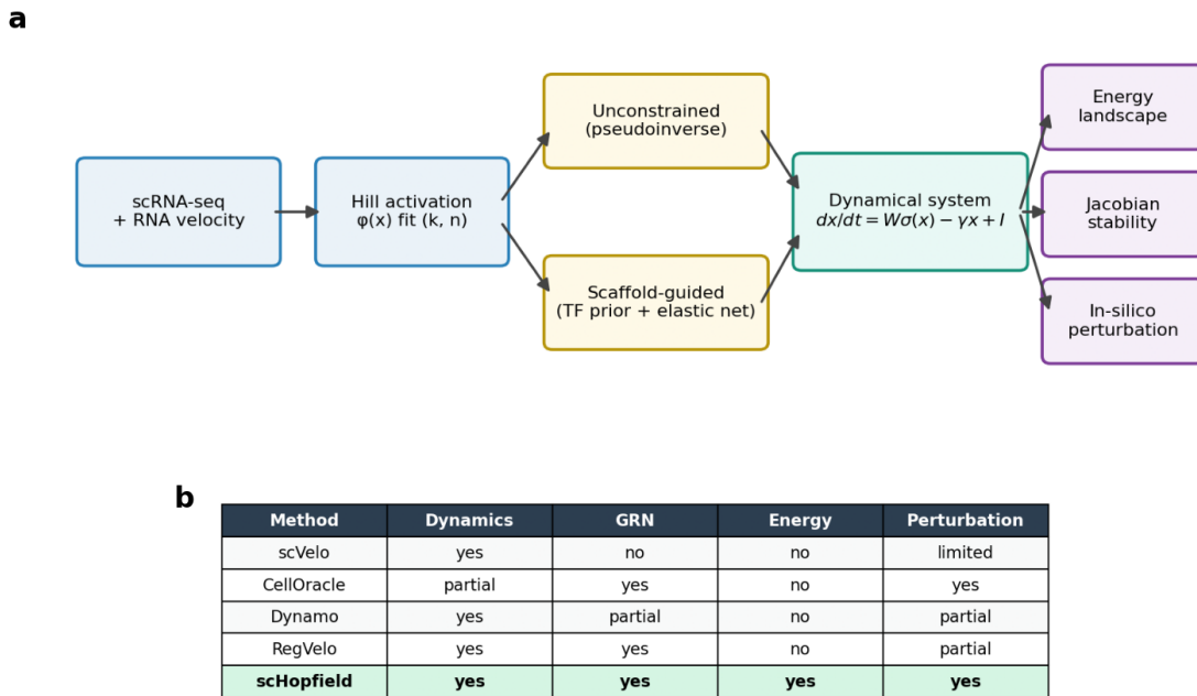
Figure 1: Overview of scHopfield. Single-cell expression and RNA velocity are used to fit Hill activation functions; a cell-type-specific interaction matrix is inferred either unconstrained (pseudoinverse) or scaffold-guided; the resulting dynamical system yields an energy landscape, Jacobian-based stability, and in-silico perturbation.
