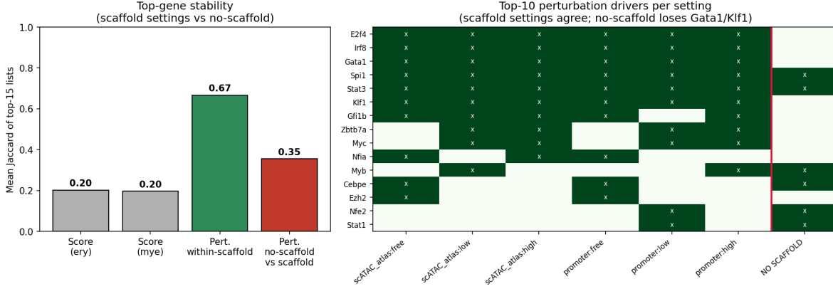
Figure 4: Driver identification is robust to network and regularization choices. Perturbation-based drivers are stable across two base networks and three scaffold-regularization regimes (Jaccard 0.67) while the static network score is unstable (0.20); the no-scaffold pseudoinverse is an outlier that loses canonical drivers (benchmarks M5, M6).
