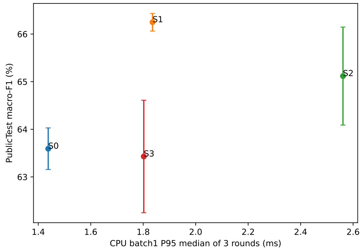
90 epochs CE; 3 seeds; mean \pm sample SD (descriptive)
