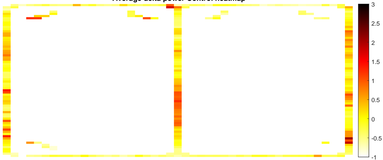
Average delta power Control heatmap
