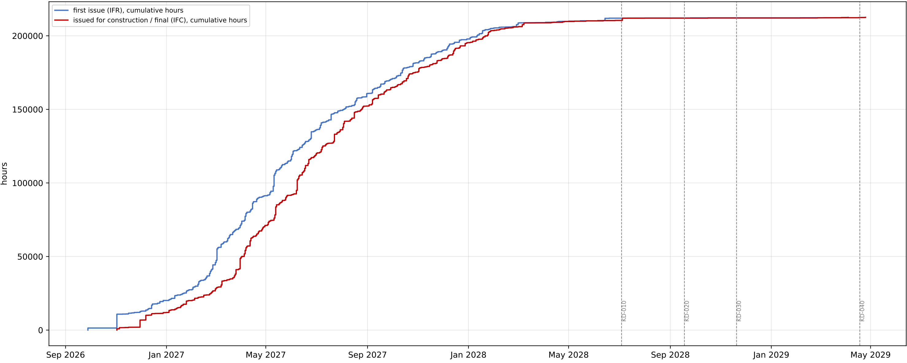
Engineering progress curve - 2238 documents, 212,536 h (step at NTP: 180 tender-stage documents, 10,757 h; supplier documents at their VDRL dates) - levelled to the discipline capacities
