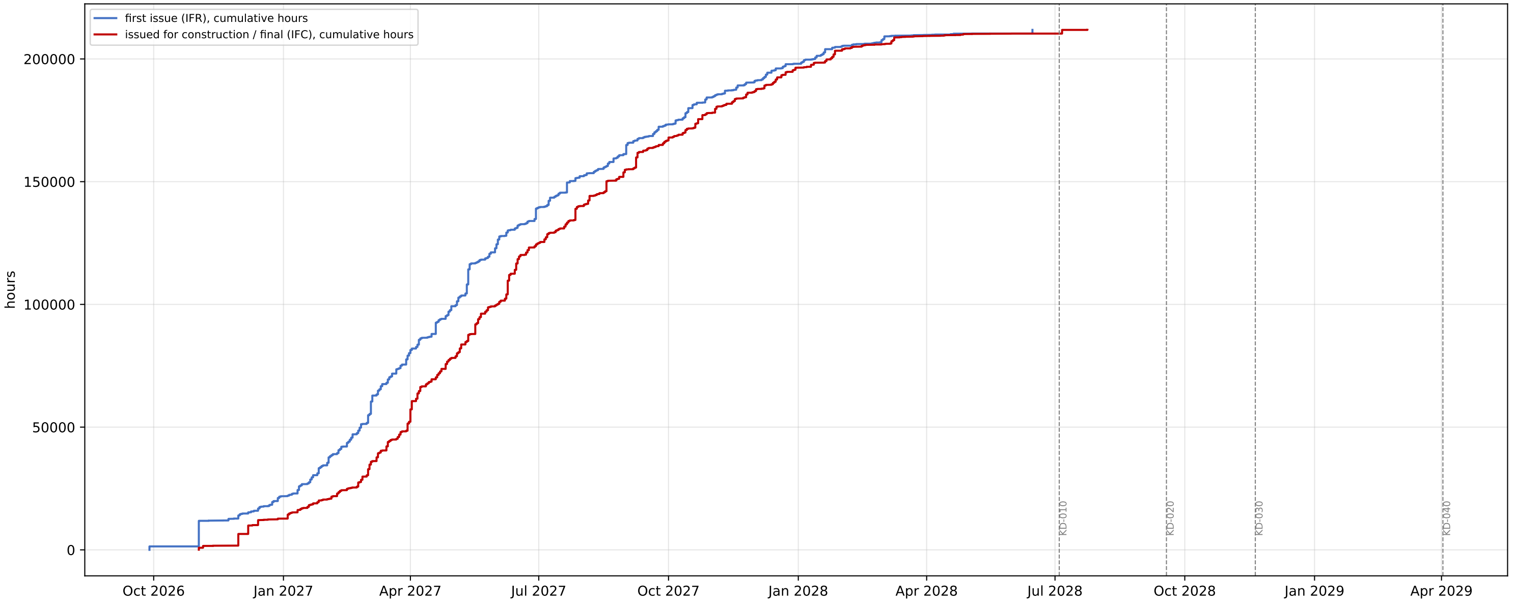
Engineering progress curve - 2208 documents, 211,845 h (step at NTP: 174 tender-stage documents, 10,413 h; supplier documents at their VDRL dates) - levelled to the discipline capacities
