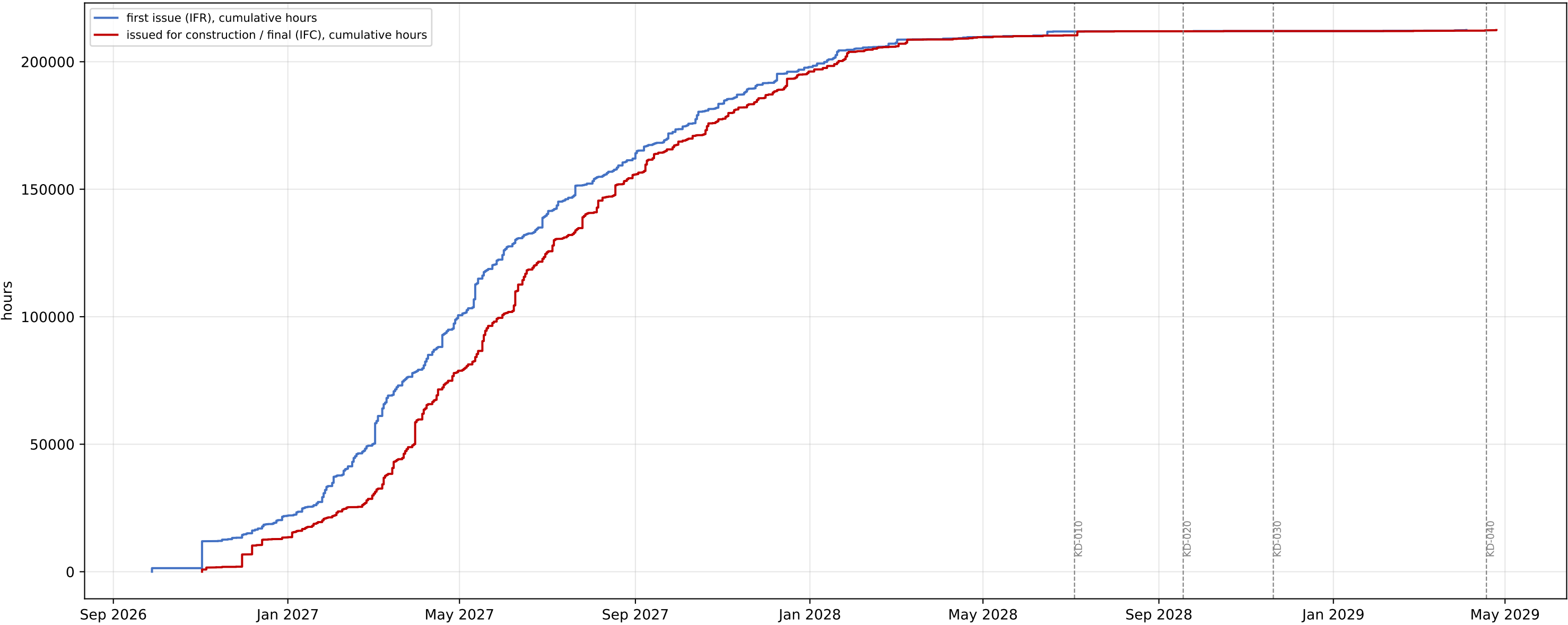
Engineering progress curve - 2237 documents, 212,424 h (step at NTP: 180 tender-stage documents, 10,697 h; supplier documents at their VDRL dates) - levelled to the discipline capacities
