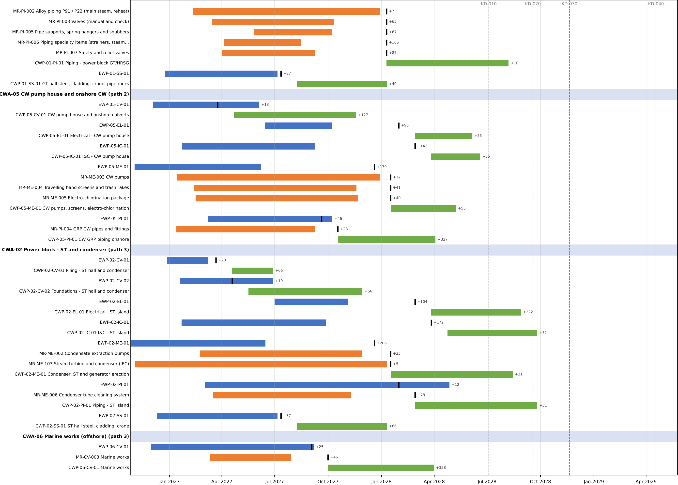
AWP timeline - EWP (blue: first document start to all IFC), PWP (orange: PO to on site), CWP (green: CPM) | = first need (EWP: CWP start - lead; progressive documents later); numbers = float in working days (EWP: smallest document float); red = late [page 3]
