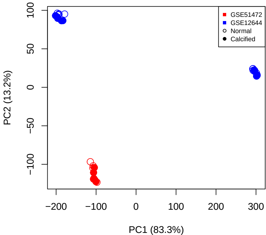
Before ComBat
