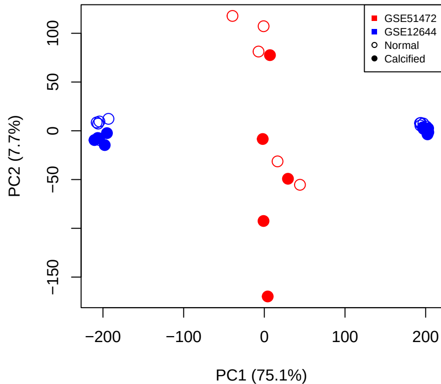
After ComBat
