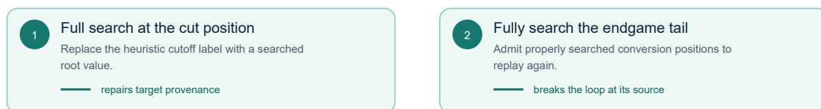
Late-game target poisoning feedback loop and its two-stage repair
