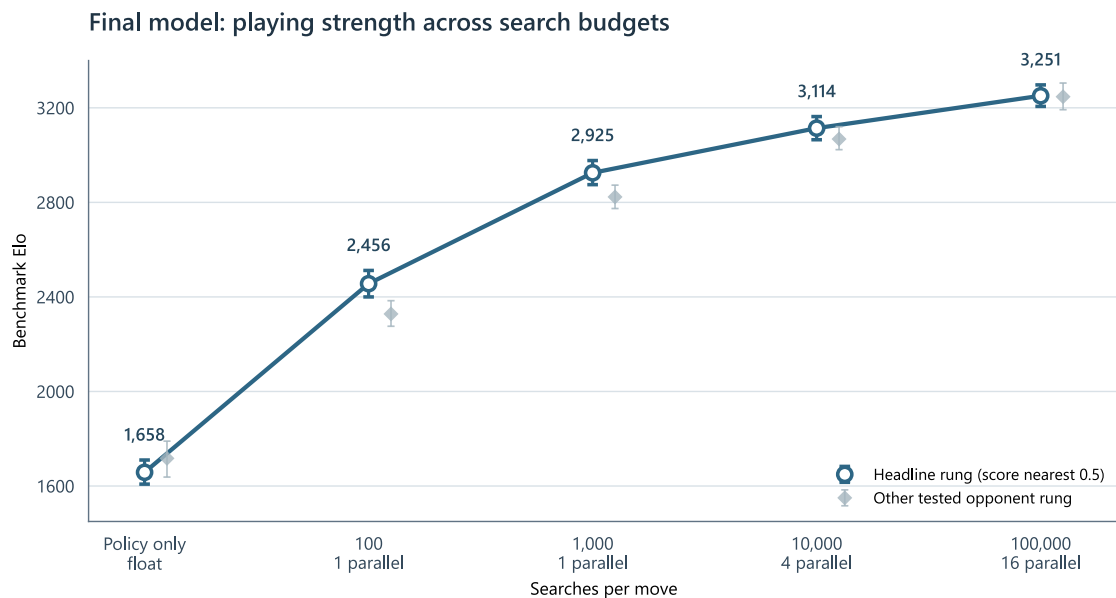
Figure 9: The connected points use the opponent rung with score nearest 0.5; pale diamonds show the other measured rung at each budget. Vertical bars are the reported 95% confidence intervals. The categorical horizontal axis keeps policy-only play visible alongside the searched conditions; it does not imply equal compute spacing. Policy-only uses the float export, while searched points use INT8 TensorRT. The parallel-search count also changes with budget, so this is a measured operating curve rather than an isolated node-budget experiment.
