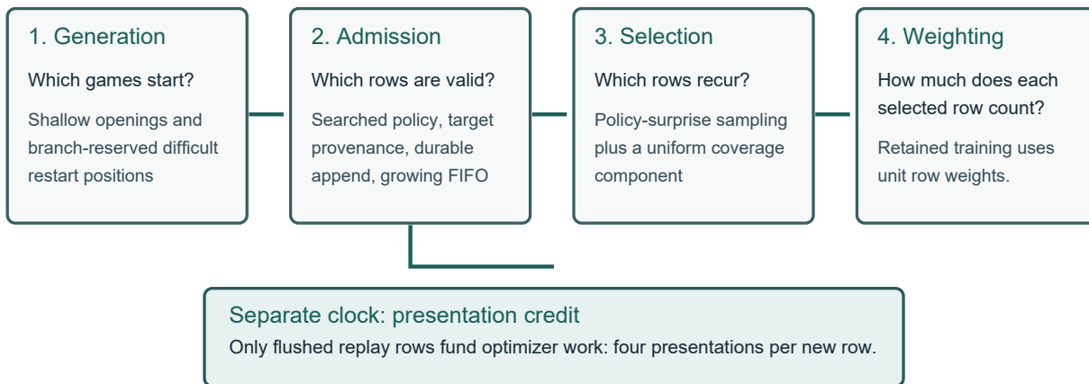
Figure 3: The retained curriculum changes where games start and which valid positions recur, but leaves admitted rows at unit loss weight. The separate presentation-credit ledger allows optimizer work only after replay append and flush; a sampled row is not the same unit as a newly generated row.
