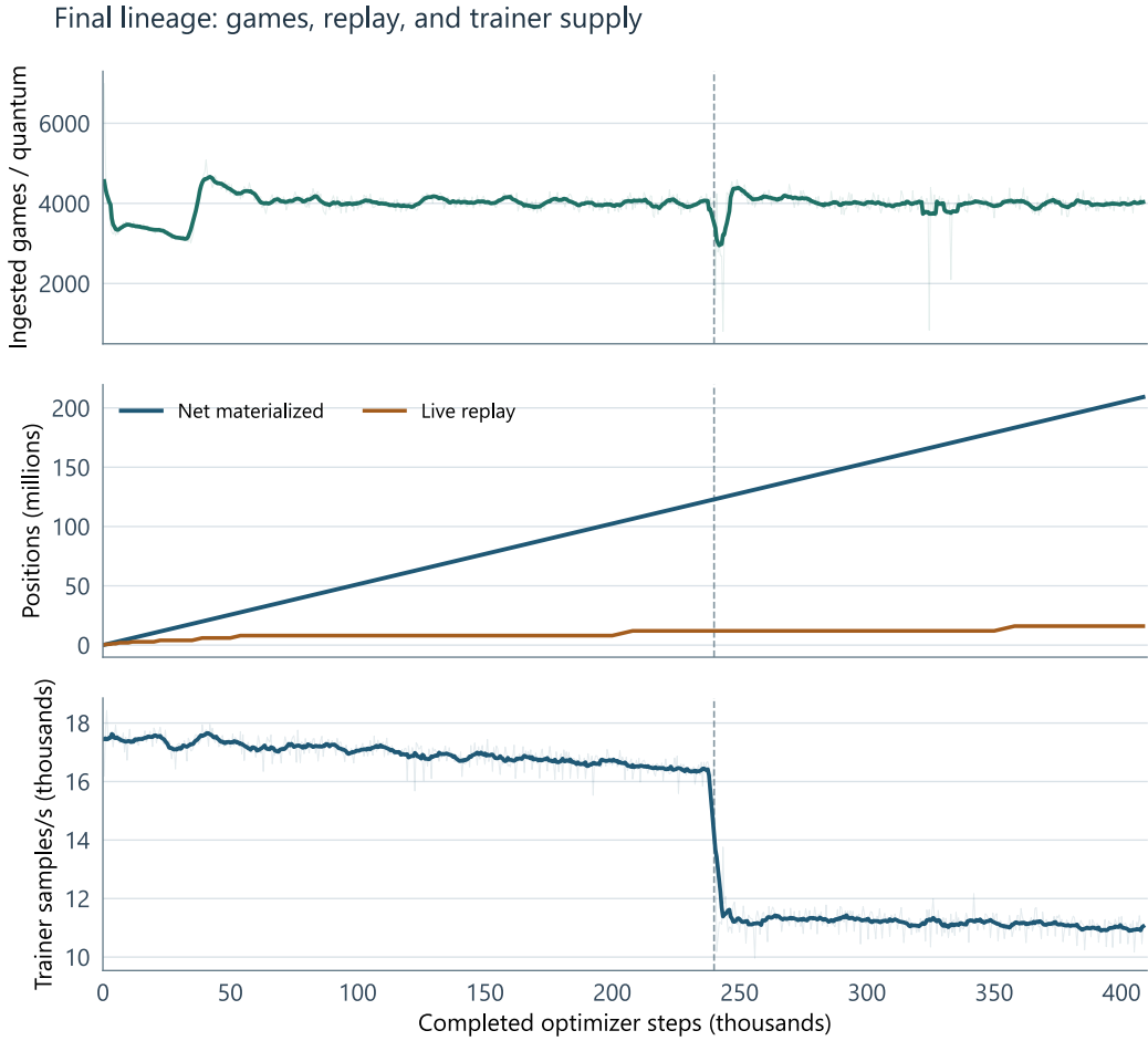
Figure A.2: Per-quantum completed games, net materialized positions, live replay occupancy, and training samples per second share an optimizer-step axis. The small model’s median measured trainer throughput was 16,977 samples/s across 480 quanta; the medium model’s was 11,194 across 337. Model shape, schedule, and concurrent workload differ, so the gap is not an isolated model-size effect.
