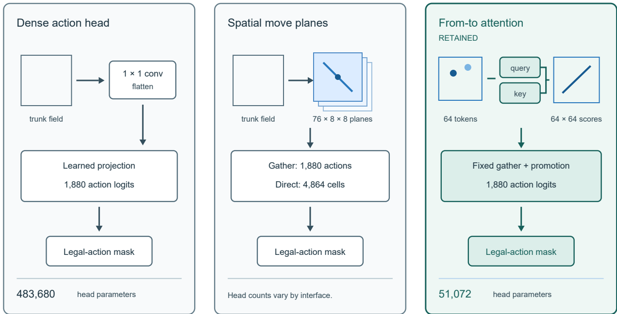
Figure 4: Policy representation changes the learned output geometry. Dense heads learn an action-sized projection, move-plane heads preserve spatial move types, and the retained from-to head scores square pairs before a fixed gather. The parameter counts are from the same controlled convolutional-trunk comparison; no count is shown for the plane family because its implementations and external interfaces differed. The diagram is architectural, not a playing-strength comparison.
