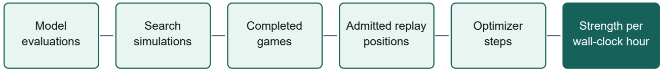
Figure 6: The denominator changes at each boundary. Model evaluations and search simulations describe local service capacity; completed games and admitted rows determine training supply; only the final stage measures the playing-strength gain per unit wall-clock time.
