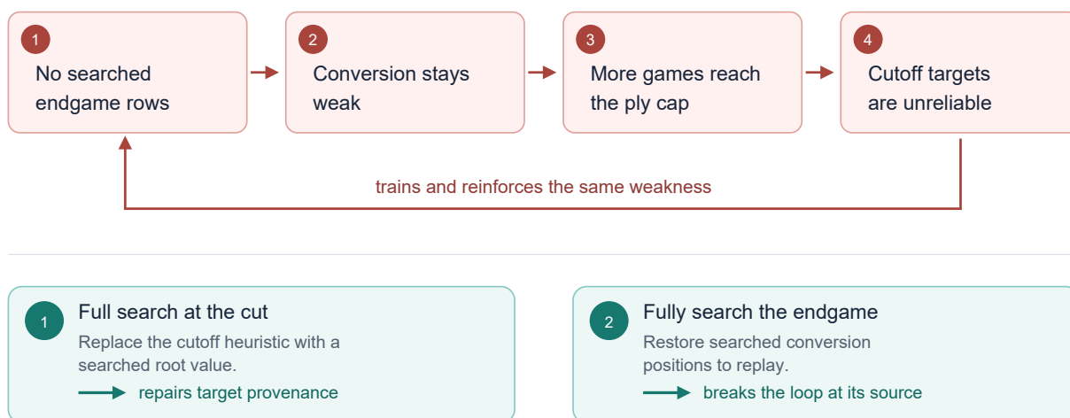
Figure 7: A searched cutoff value improves labels for unfinished games; restoring fully searched endgames also returns the examples needed to learn conversion.
