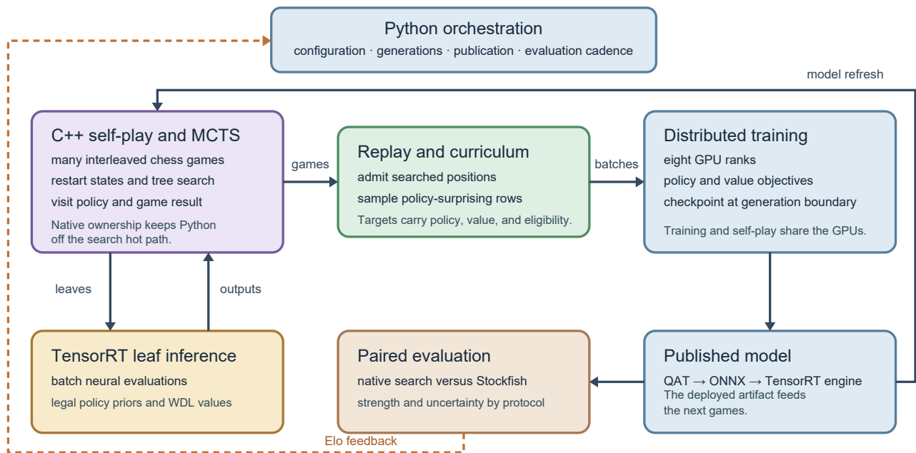
Figure 1: A published model guides batched native self-play; searched positions become replay targets for the trainer. Paired evaluation measures the published checkpoint and informs model-promotion decisions.
