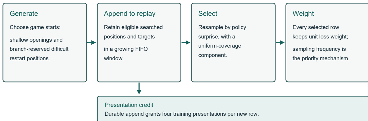
Figure 3: Starting positions shape the games that are played. Their searched positions enter replay, where sampling determines which examples the learner revisits. New examples also set the pace of optimizer updates.
