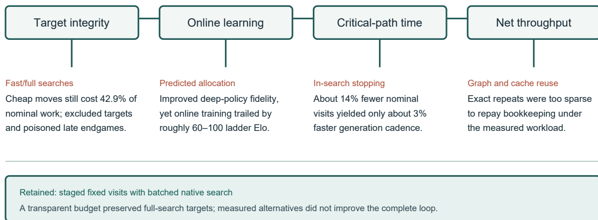
Figure 2: Why the search alternatives were not retained. Fast/full search discarded useful targets; predicted allocation improved policy agreement but weakened learning; stopping saved search without much faster training; and exact graph or cache reuse saved too little work to repay its overhead.
