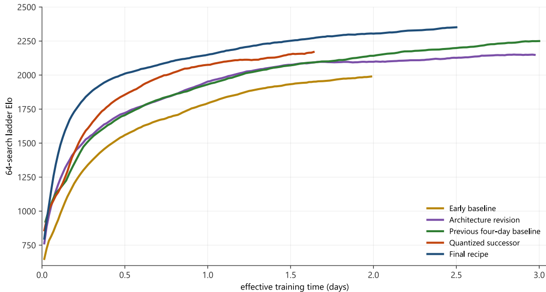
Figure 8: Smoothed 64-search training ladders across five chess campaigns. The final curve ends at 2.5 days and the preceding baseline at 3.0 days; the matched comparison uses a common rating calculation.
