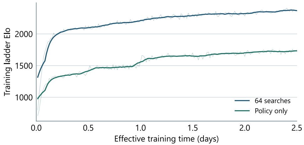
Figure A.5: Policy-only and 64-search training-ladder ratings over the final 2.5-day window. Faint traces show individual evaluations and solid curves average eleven evaluations. Both improve over training; Table 1 reports the separate final matches.
