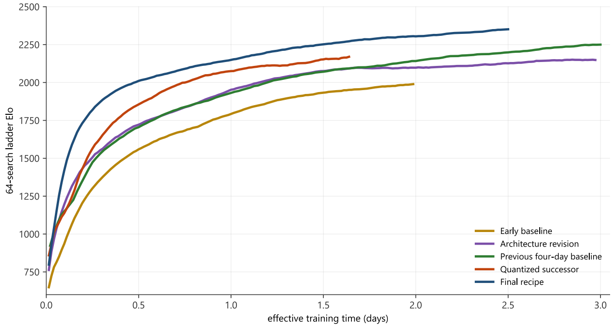
Figure 11: Smoothed 64-search training ladders across five chess campaigns. The final curve ends at 2.5 days and the preceding baseline at 3.0 days; the matched comparison uses a common rating calculation.
