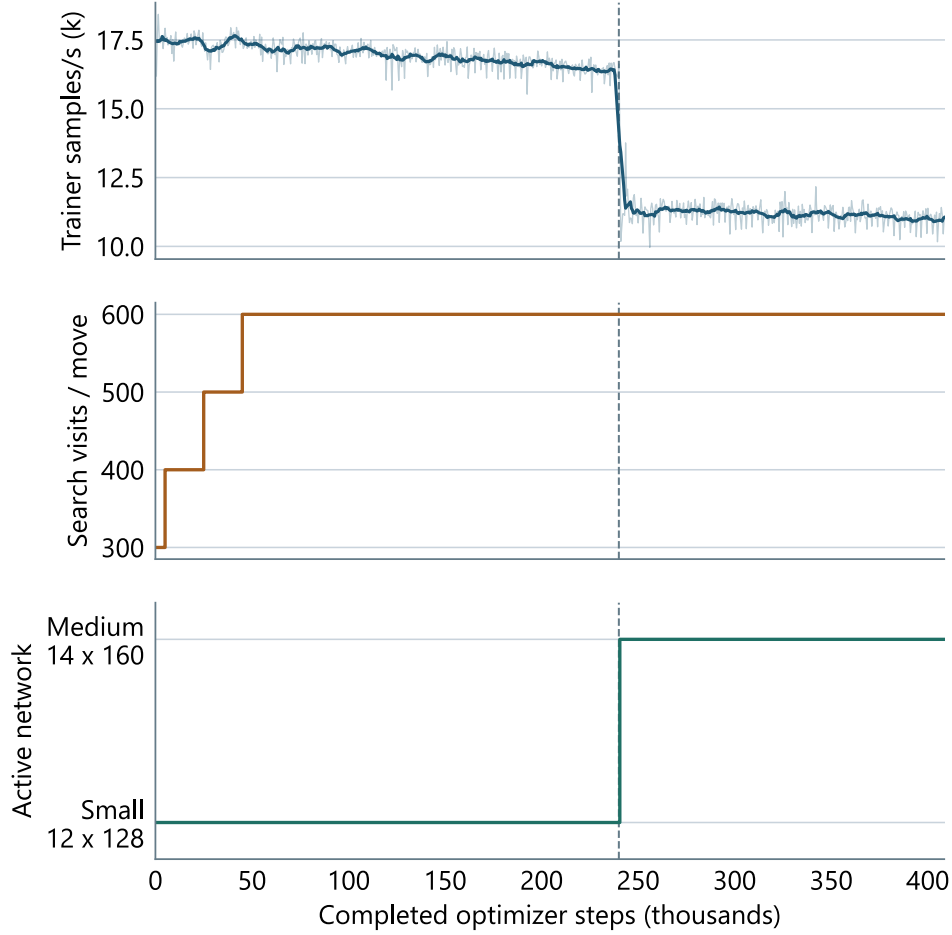
Figure A.6: Trainer throughput, self-play search budget, and active network. The small-to-medium transition coincides with lower trainer throughput. The plotted training sequence increases search from 300 to 600 visits; the configured 800-visit stage lies beyond the selected checkpoint.
