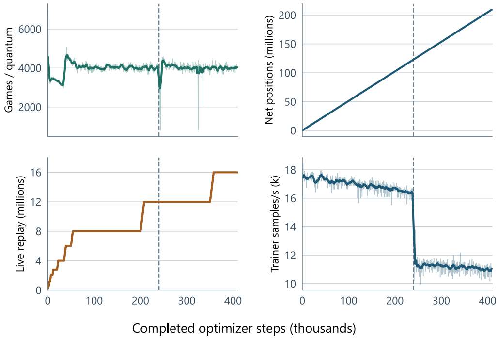
Figure A.2: Training volume and throughput on a common optimizer-step axis: completed games per quantum, cumulative net materialized positions, live replay occupancy, and training samples per second. The run completed 3,249,647 games and materialized 209.15 million net positions, with 16 million rows retained at selection. Median trainer throughput was 16,977 samples/s across 480 small-model quanta and 11,194 across 337 medium-model quanta under their respective schedules and concurrent workloads.
