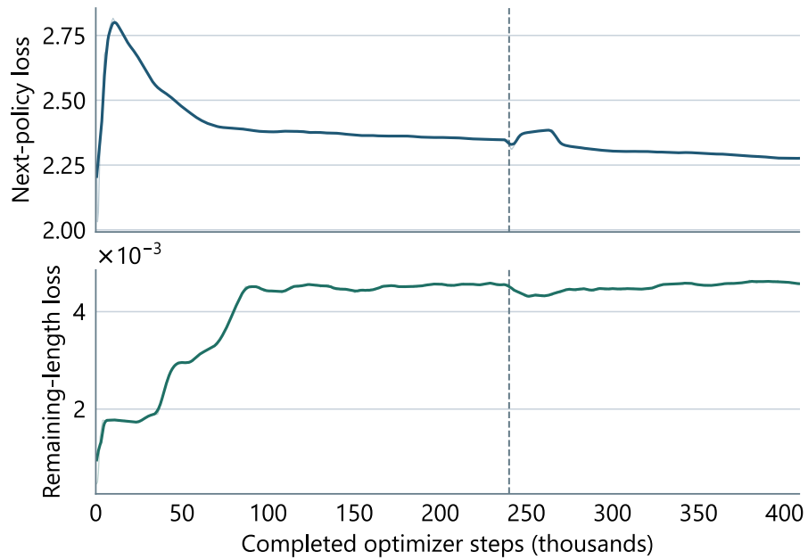
Figure A.3: Next-policy and remaining-game-length losses on separate scales. Faint traces show recorded values; solid curves show 11-quantum moving averages. The dashed line marks the small-to-medium transition, as in the remaining optimizer-step plots.
