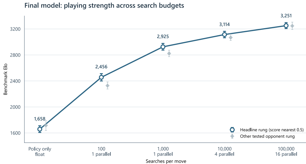
Figure 7.2: The connected points use the opponent rung with score nearest 0.5; pale diamonds show the other measured rung at each budget. Vertical bars are the reported 95% confidence intervals. The categorical horizontal axis keeps policy-only play visible alongside the searched conditions; it does not imply equal compute spacing. Policy-only uses the float export, while searched points use INT8 TensorRT. The parallel-search count also changes with budget, so this is a measured operating curve rather than an isolated node-budget experiment.
