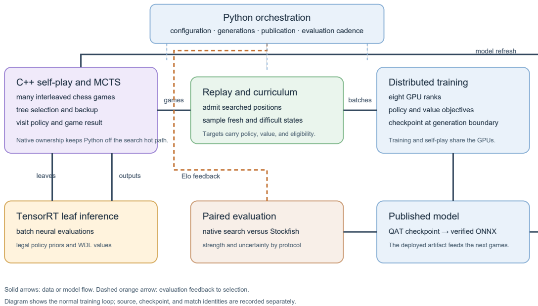
Figure 3.1. A published model returns to batched native self-play; searched positions become replay targets for the trainer. Paired evaluation measures the published checkpoint and feeds selection decisions back to Python. The diagram shows ownership and data flow, not the number or scheduling of every worker.
