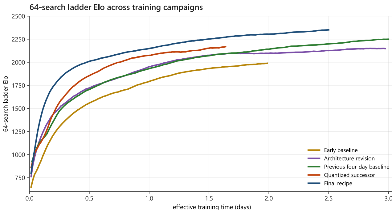
Figure 7.1: Each curve uses the bias-corrected 0.95 exponential moving average used by the project's earlier training-dynamics plots. The final recipe is cut at 2.5 days and the previous four-day baseline at 3.0 days. The figure is descriptive; the +74.1 Elo claim comes from the matched-estimator plateau audit rather than from subtracting its displayed endpoints.
