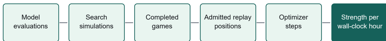
Figure 5.1: The denominator changes at each boundary. Model evaluations and search simulations describe local service capacity; completed games and admitted rows determine training supply; only the final stage measures the playing-strength gain per unit wall-clock time.
