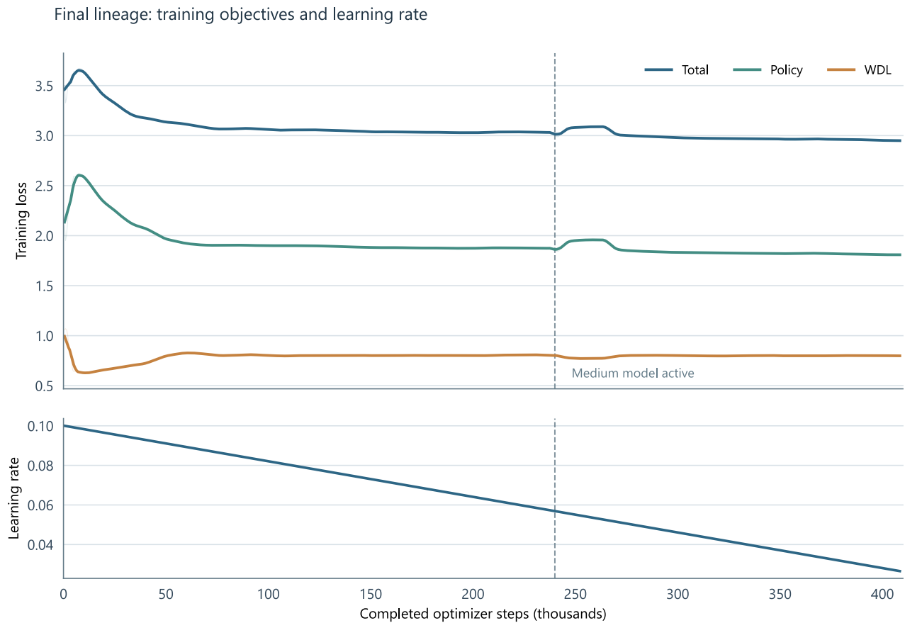
Figure A.1: Total, policy, and WDL training losses are shown with an 11-quantum moving average over faint raw observations. The dashed line marks the small-to-medium active-model transition at 240,000 optimizer steps. Loss levels across model stages are optimization diagnostics, not paired playing-strength measurements. The active learning rate fell from about 0.10 to 0.0266 by selection.
