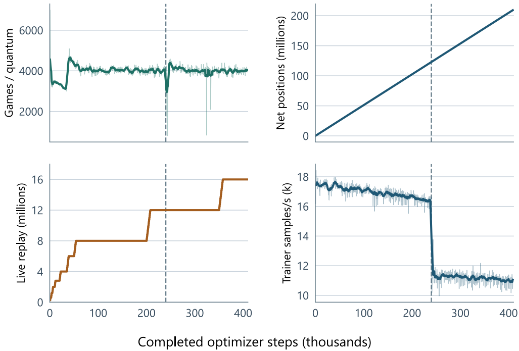
Figure 12: Training volume and throughput on a common optimizer-step axis. Panels show completed games per training block, cumulative materialized positions, live replay occupancy, and trainer throughput. Replay capacity increases in steps, while the small-to-medium transition coincides with lower trainer throughput.
