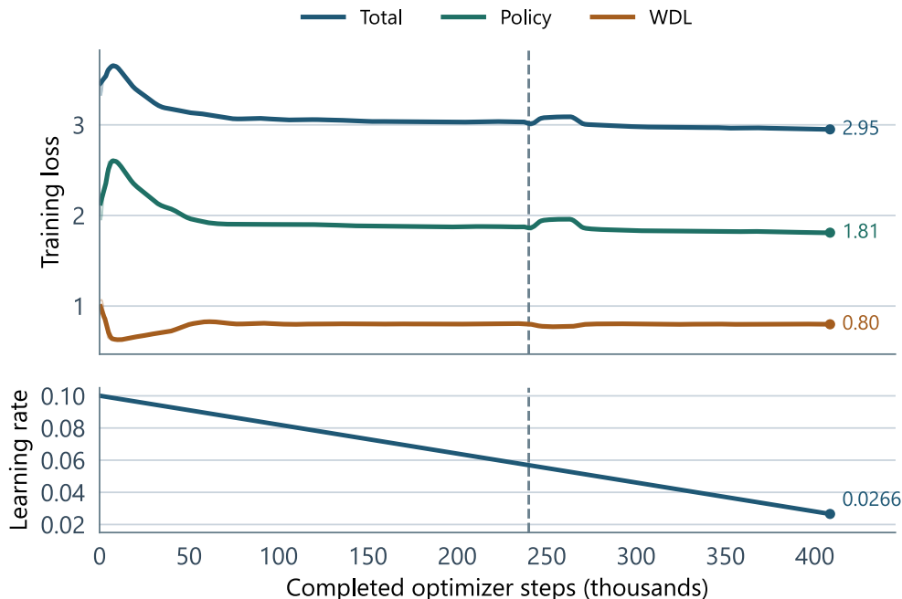
Figure A.1: Training losses and learning rate. Raw losses are overlaid with 11-quantum moving averages; the dashed line marks the small-to-medium transition at 240,000 optimizer steps. From 300,000 steps to selection, total loss decreases from approximately 2.98 to 2.95 while WDL loss remains near 0.80. The learning rate declines from approximately 0.10 to 0.0266. Labels identify the final values.
