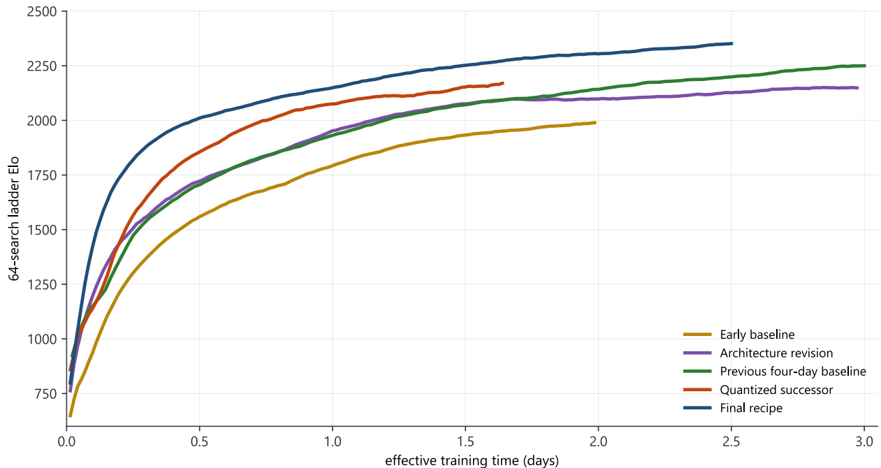
Figure 11: Smoothed 64-search training ladders across five chess campaigns. The final curve ends at 2.5 days and the preceding baseline at 3 days. Appendix B specifies the windows and the common-estimator plateau comparison.
