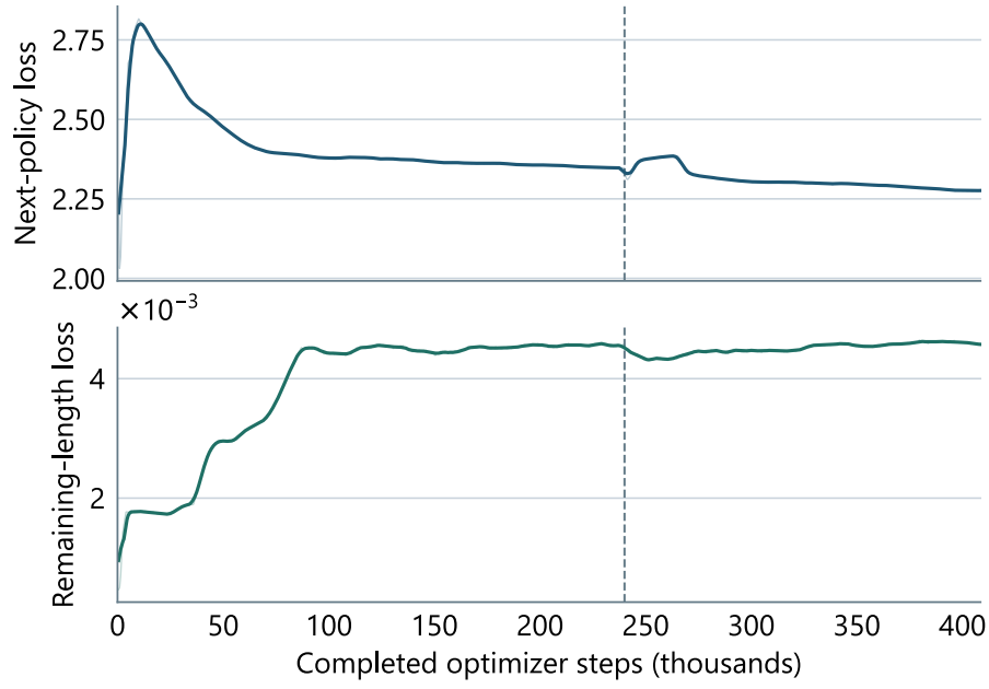
Figure A.2: Next-policy and remaining-game-length losses on separate scales. Faint traces show recorded values; solid curves show 11-quantum moving averages. The dashed line marks the small-to-medium transition, as in the remaining optimizer-step plots.
