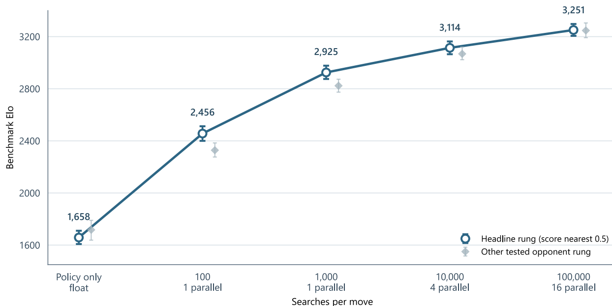
Final model: playing strength across search budgets
