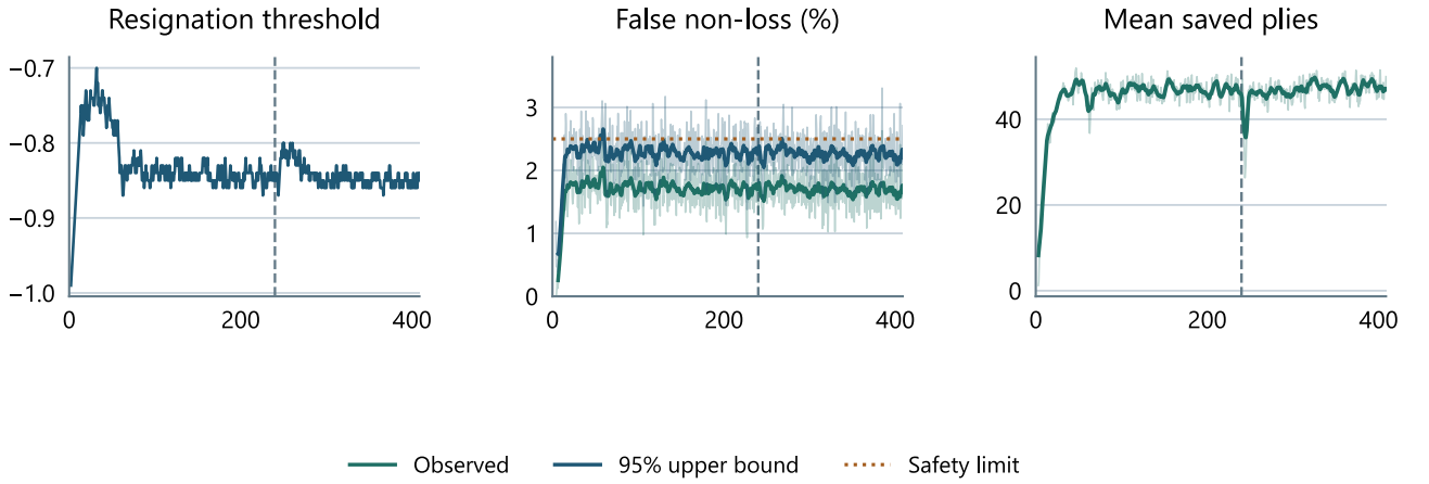
Figure 6: Resignation threshold, observed false-resignation rate and its one-sided 95% upper bound, and estimated saved plies during final training. The error panel shows periods when the resignation gate is enabled; the dotted line marks the 2.5% calibration target, including observed excursions. Saved plies are estimated from continuation games. Faint traces show raw values, with eleven-quantum averages overlaid. All horizontal axes show completed optimizer steps in thousands; the dashed vertical line marks the small-to-medium model transition.
