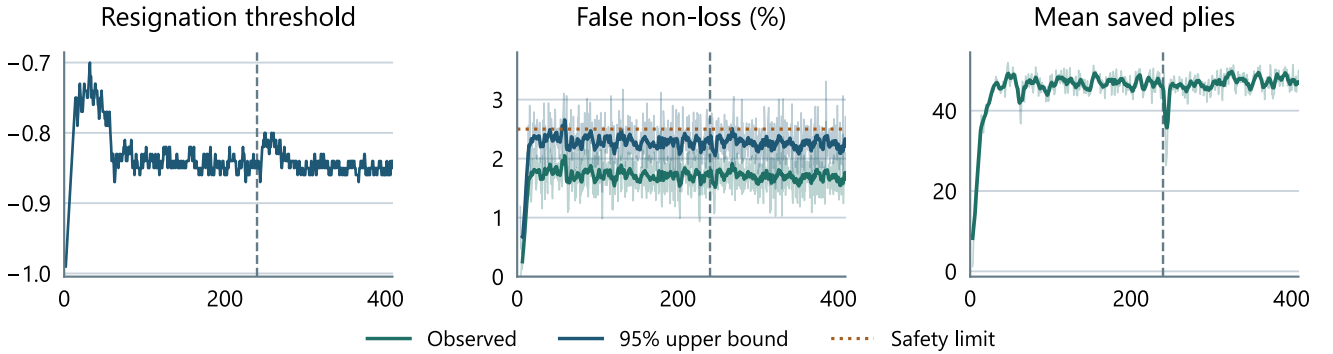
Figure 6: Resignation threshold, observed false-resignation rate and its one-sided 95% upper bound, and estimated saved plies during final training. The error panel shows periods when the resignation gate is enabled; the dotted line marks the 2.5% calibration target, including observed excursions. Saved plies are estimated from continuation games. Faint traces show raw values, with eleven-quantum averages overlaid. All horizontal axes show completed optimizer steps in thousands; the dashed vertical line marks the small-to-medium model transition.
