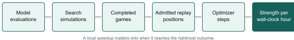
Figure 5.1: The denominator changes at each boundary. Model evaluations and search simulations describe local service capacity; completed games and admitted rows determine training supply; only the final stage measures the playing-strength gain per unit wall-clock time.
