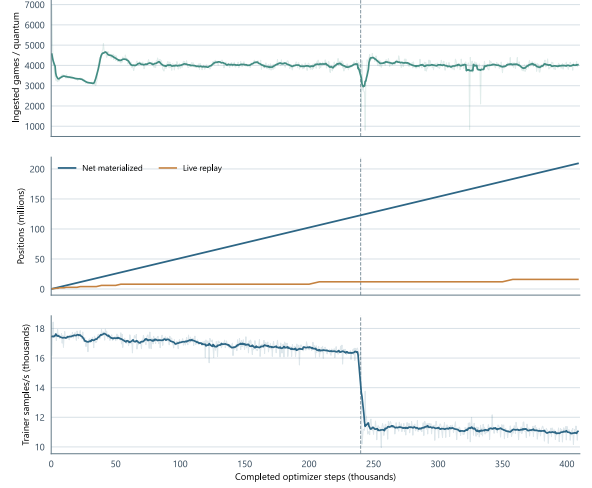
Final lineage: games, replay, and trainer supply
