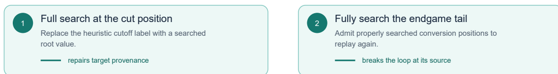
Figure 4: The cutoff repair fixes target provenance; restoring fully searched endgames breaks the feedback loop at its source.
