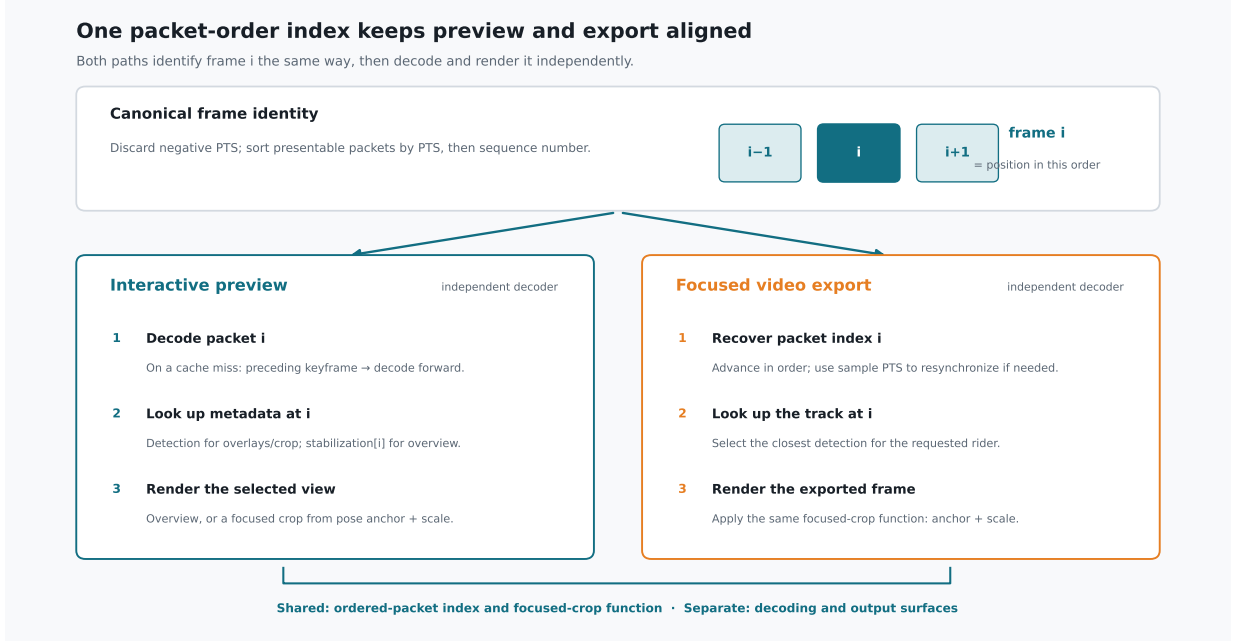
Figure 5: Preview and export decode independently but identify frame i by the same ordered-packet index. Preview seeks from a preceding keyframe; export advances its own decoder and can resynchronize by timestamp. Both use the index for track lookup, while only focused rendering shares the pose-anchor crop function.
