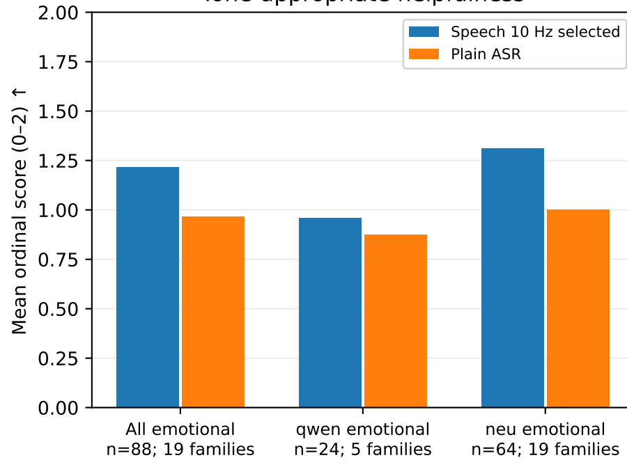
Tone-appropriate helpfulness
