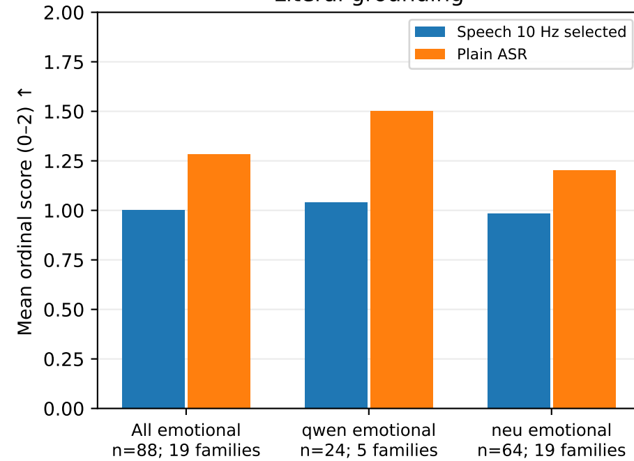
Literal grounding
