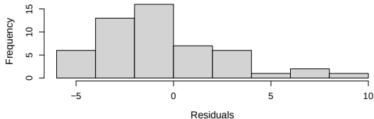
Histogram of residuals
