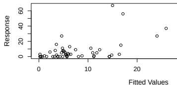
Response vs. Fitted Values
