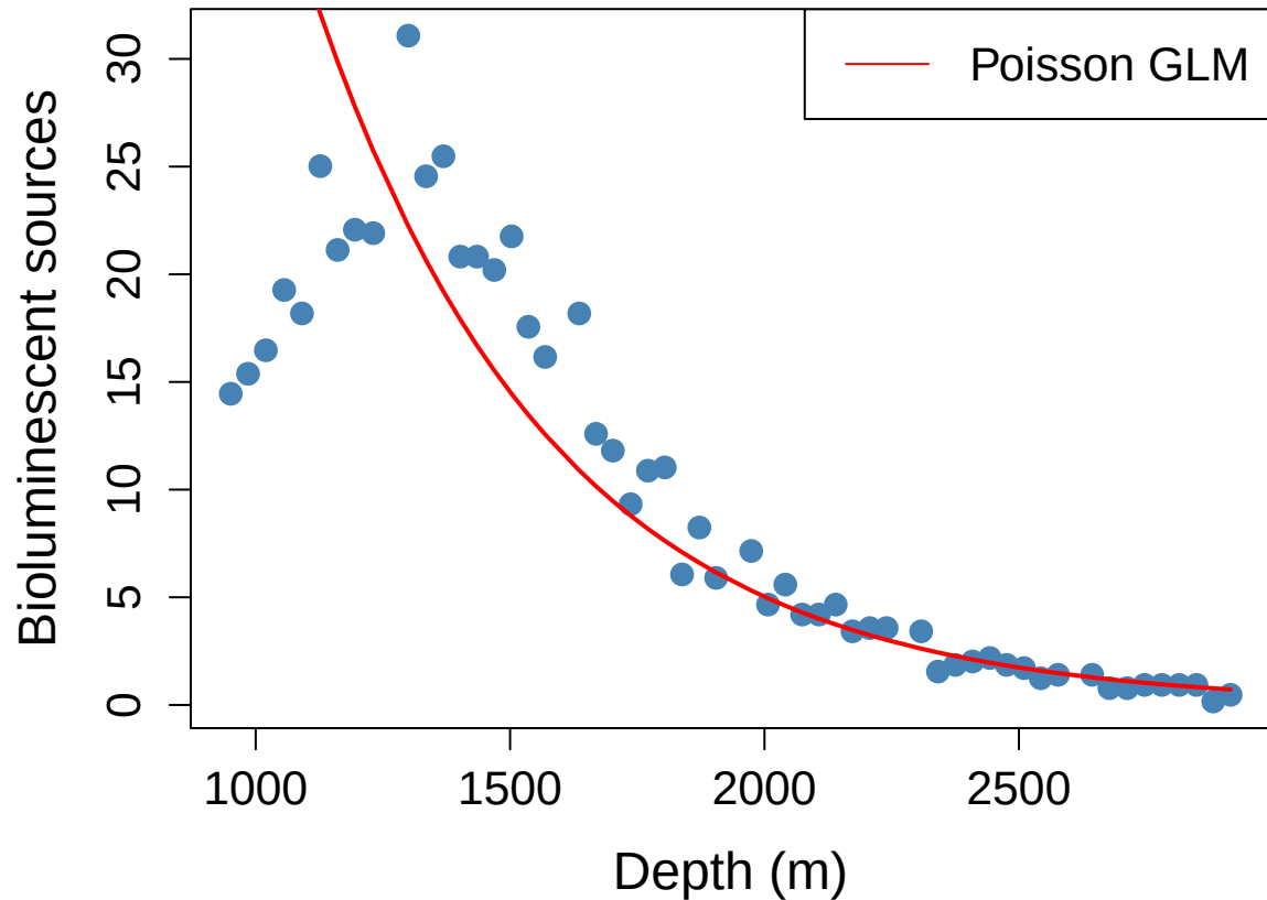
Bioluminescence vs. depth
