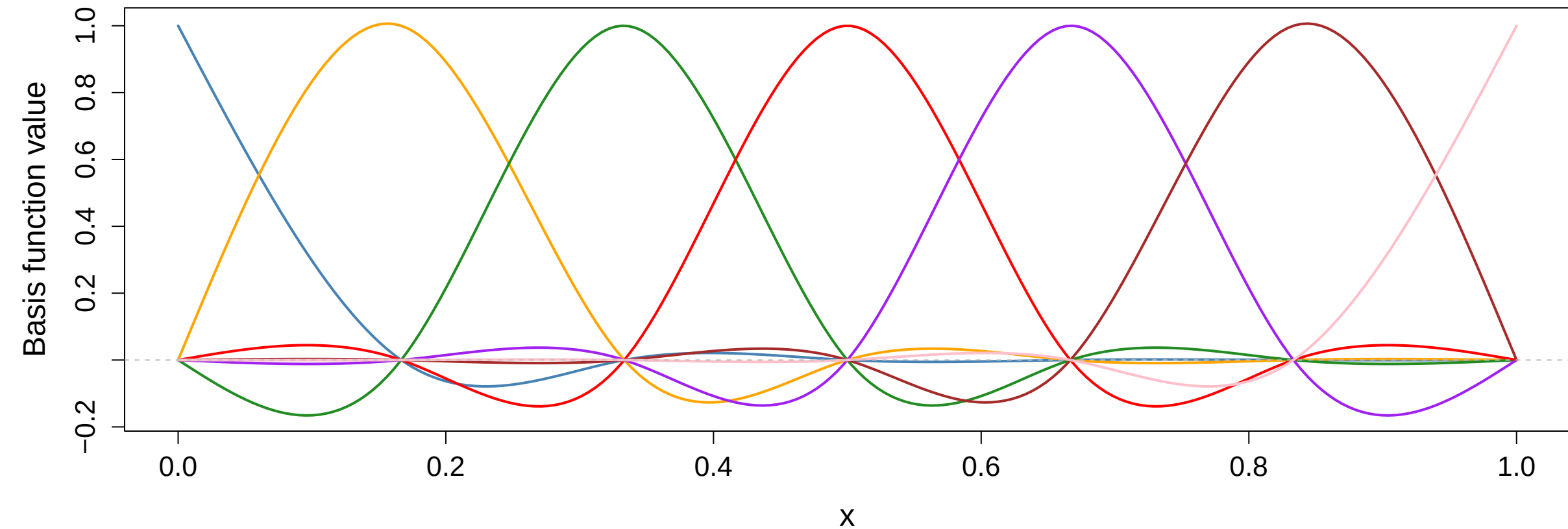
Cubic regression spline basis ( k = 7 )
