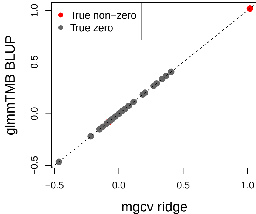
mgcv and glmmTMB agree
