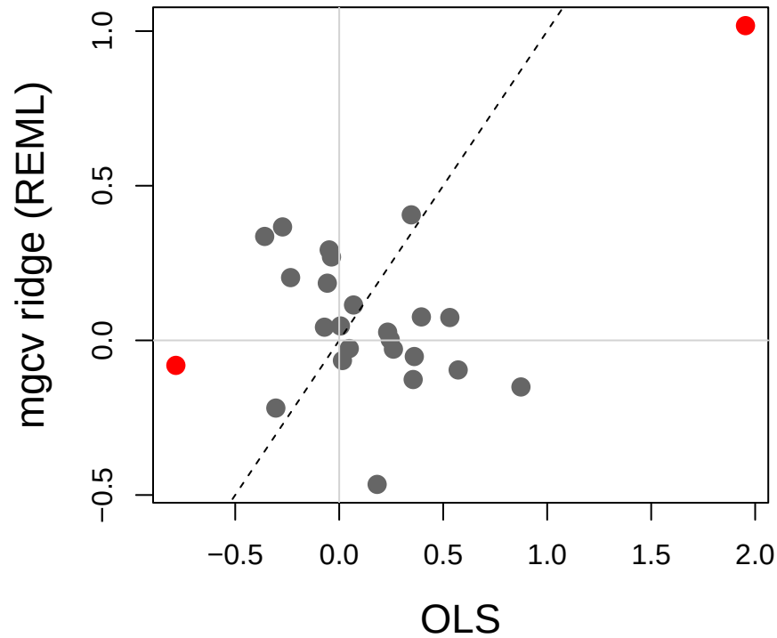
Ridge shrinks toward zero
