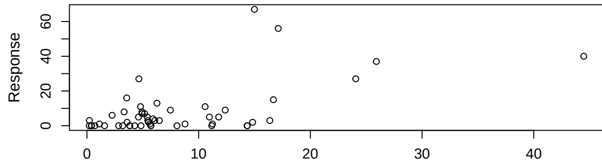
Response vs. Fitted Values
