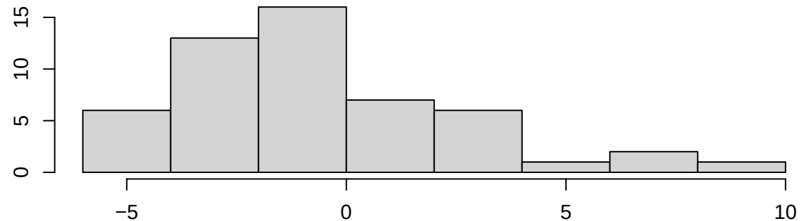
Histogram of residuals
