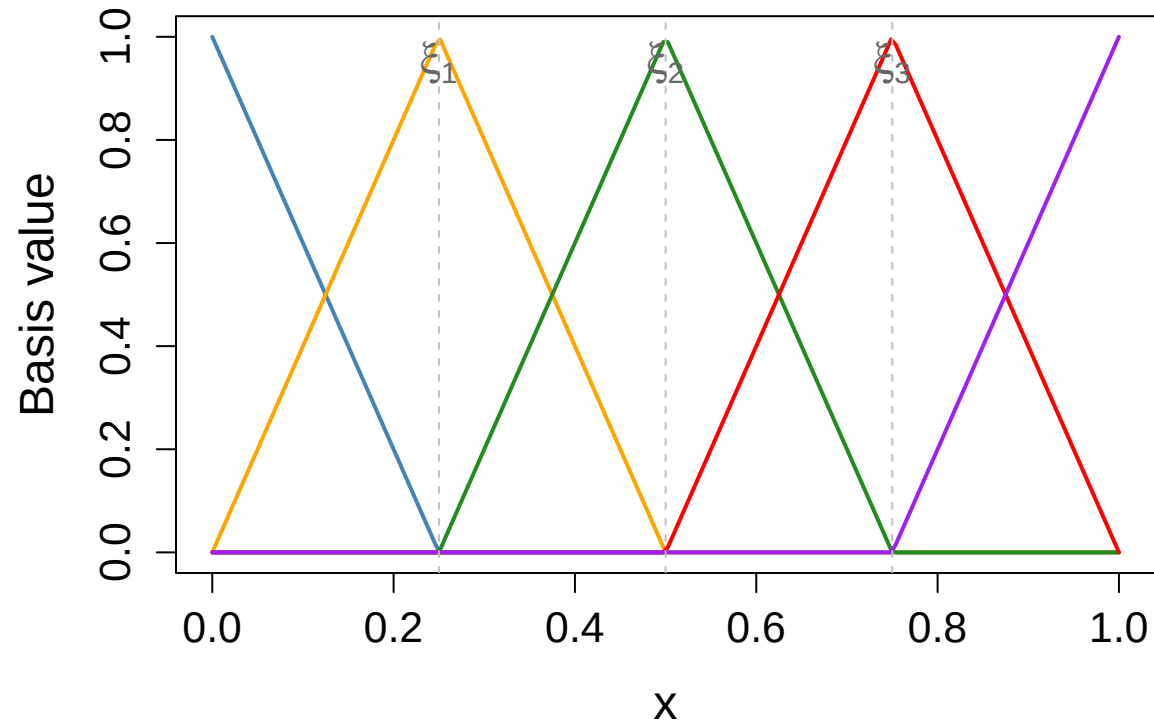
Hat functions (linear spline basis)
