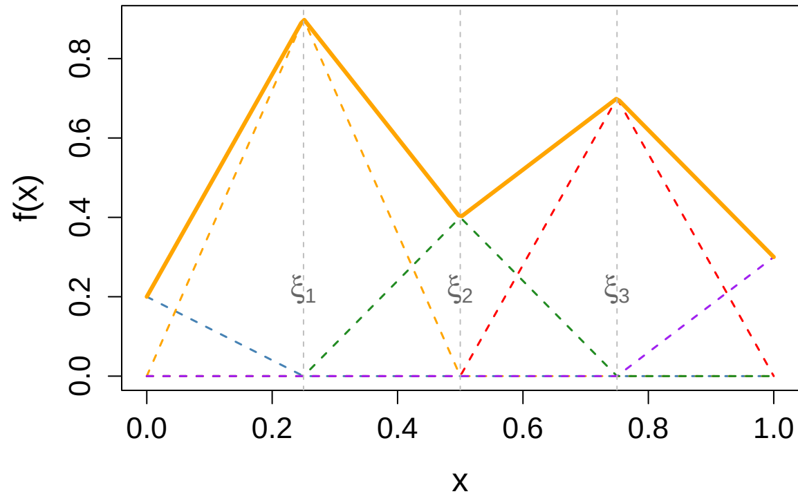
Weighted hats and their sum
