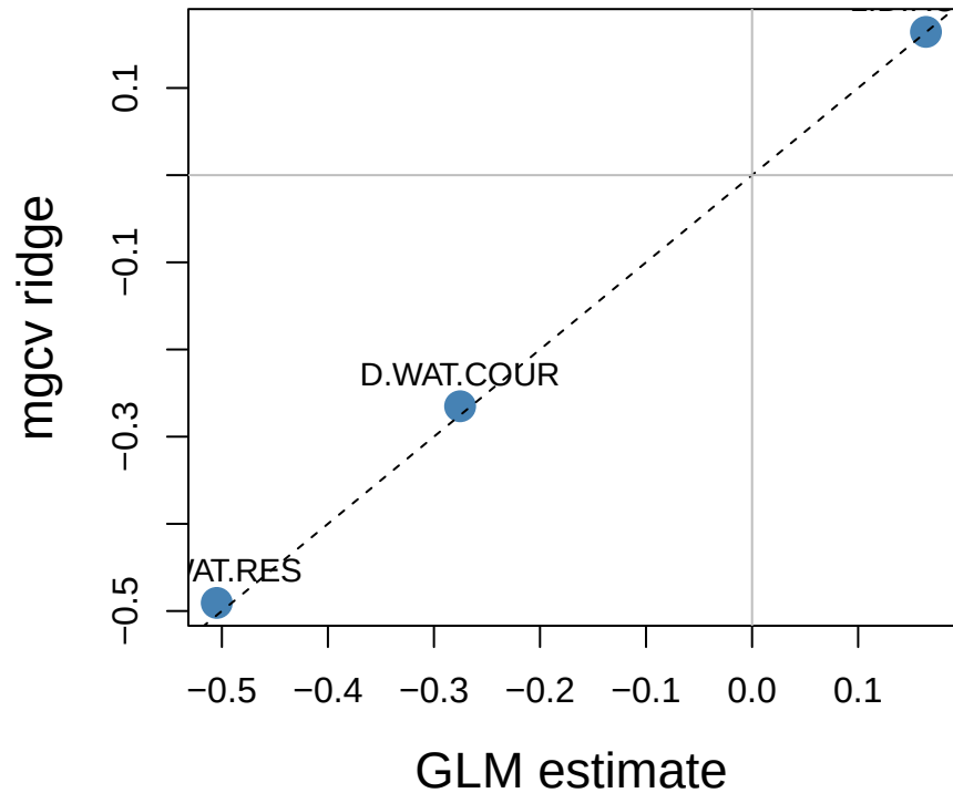
Ridge shrinks toward zero
