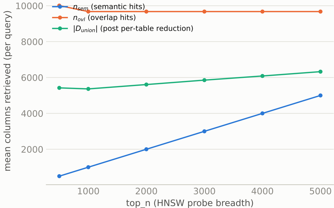
tier_100k: retrieval yield vs. top_n ( \sigma=0.30 )
