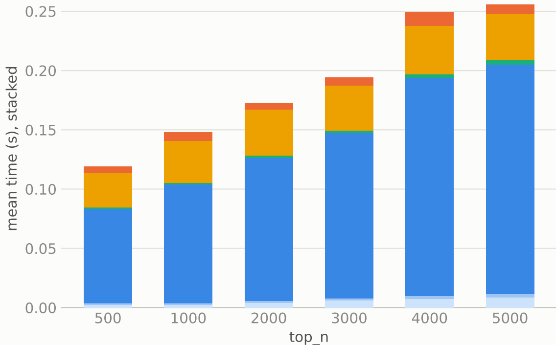
tier_10k: stage-time breakdown vs. top_n ( \sigma=0.30 , mean over \alpha, k )
