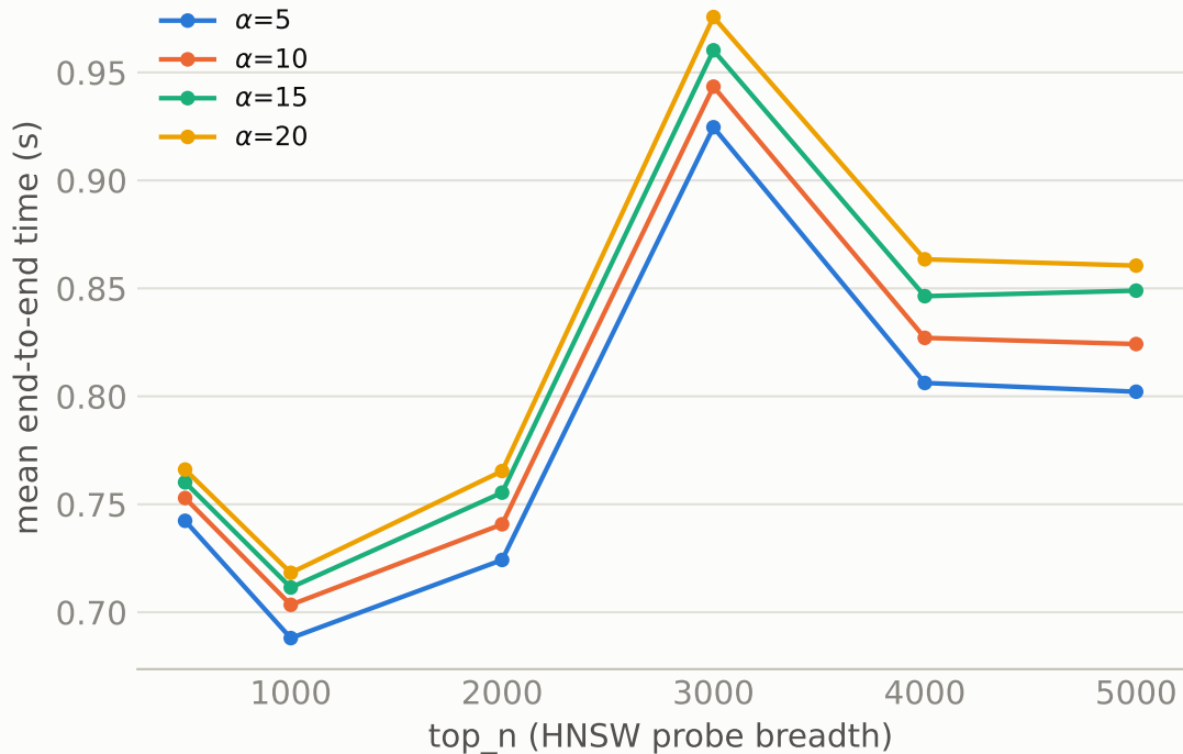
tier_100k: time vs. top_n, by \alpha ( \sigma=0.30 , union retrieval)
